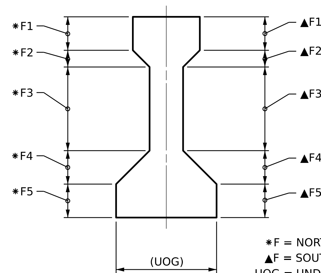
GIRDER SECTION
