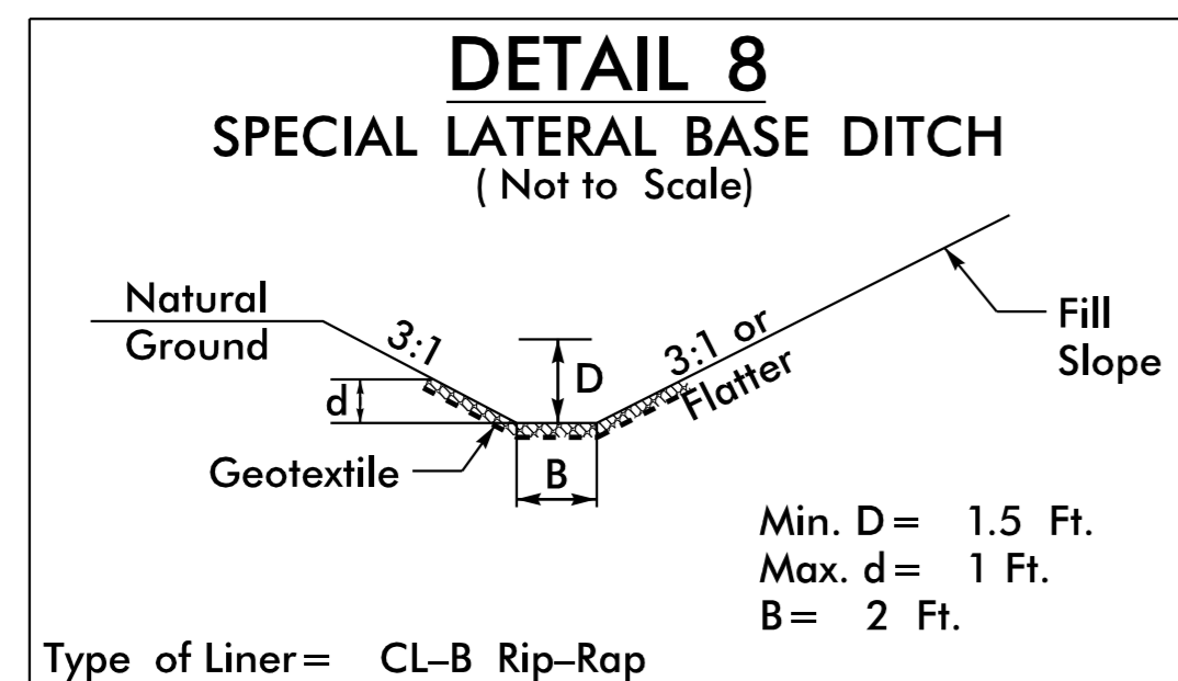
Type of Liner= CL-B Rip-Rap
