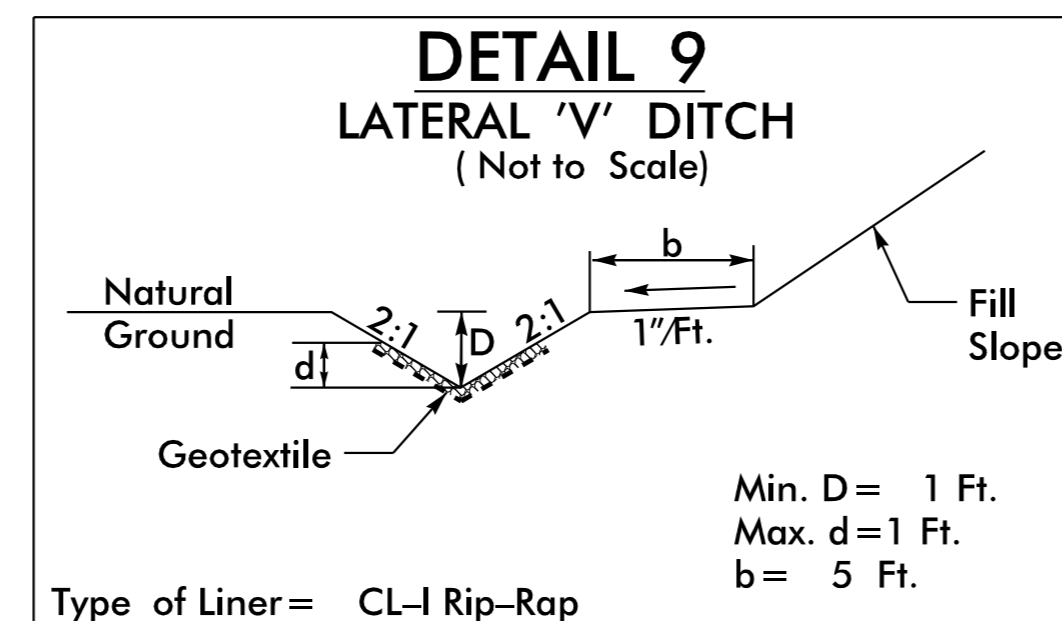
Type of Liner= CL-I Rip-Rap
