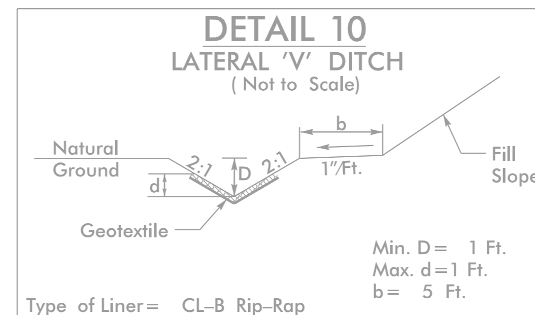
Type of Liner= CL-B Rip-Rap
