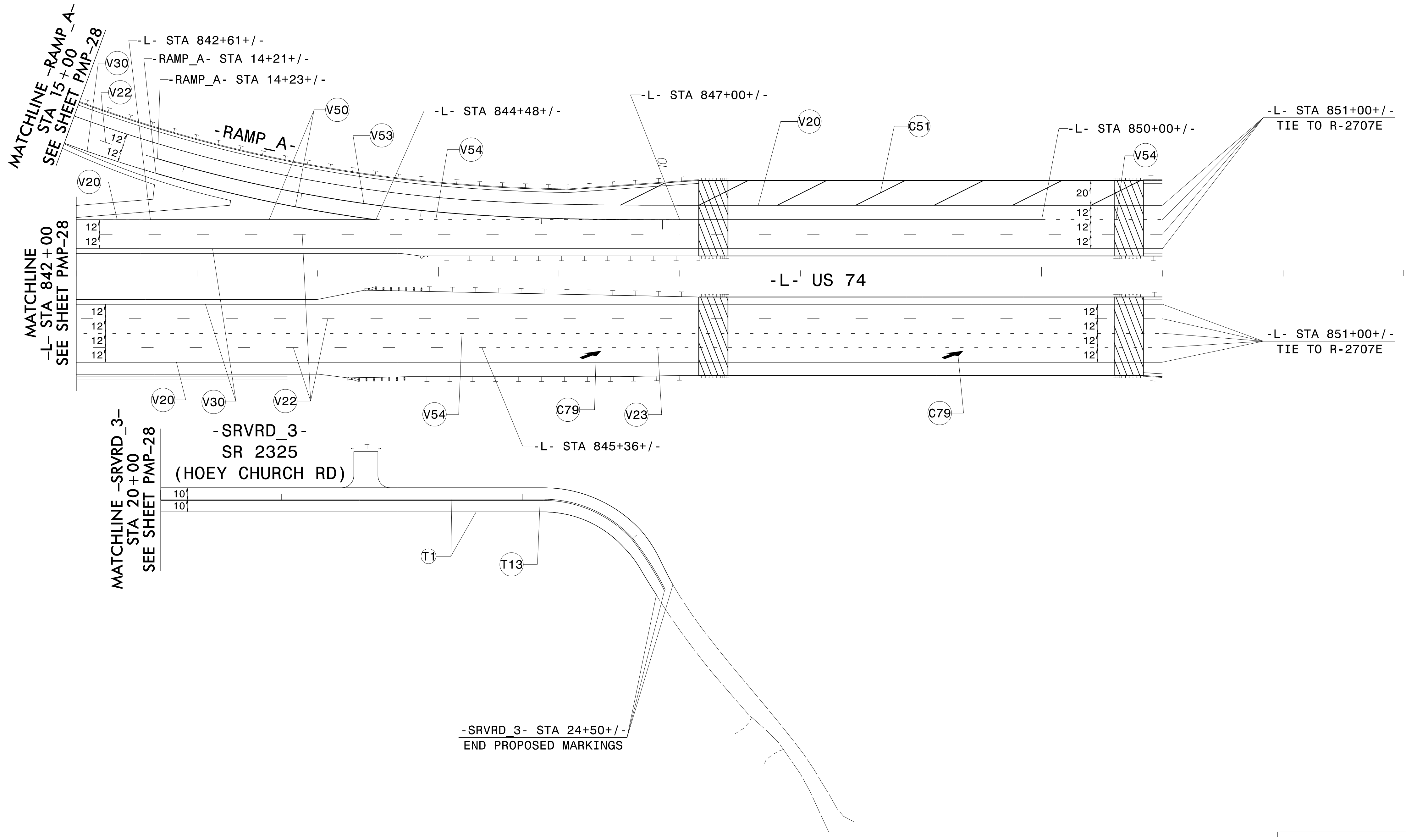
PAVEMENT MARKING DETAIL
