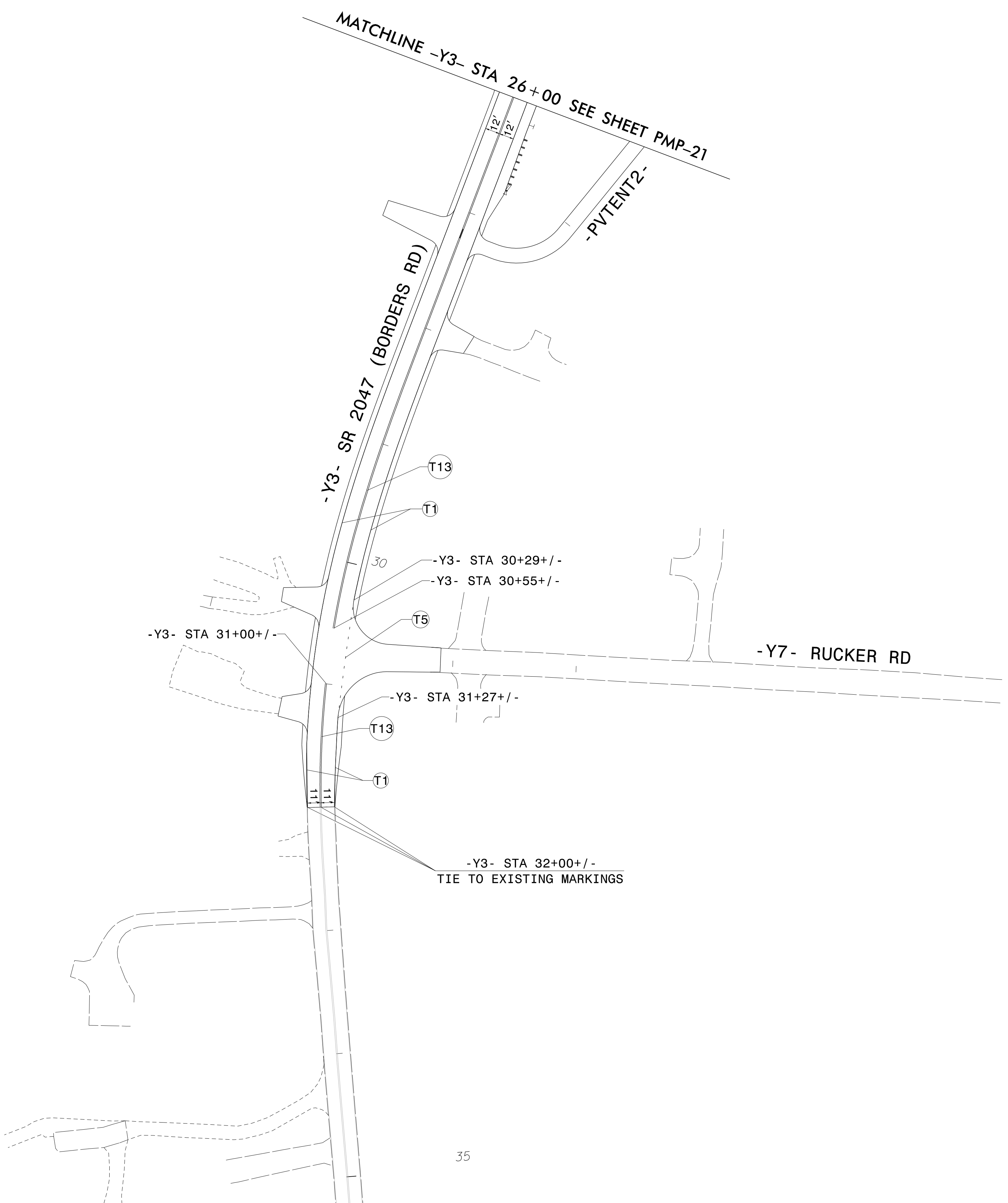
PAVEMENT MARKING DETAIL
