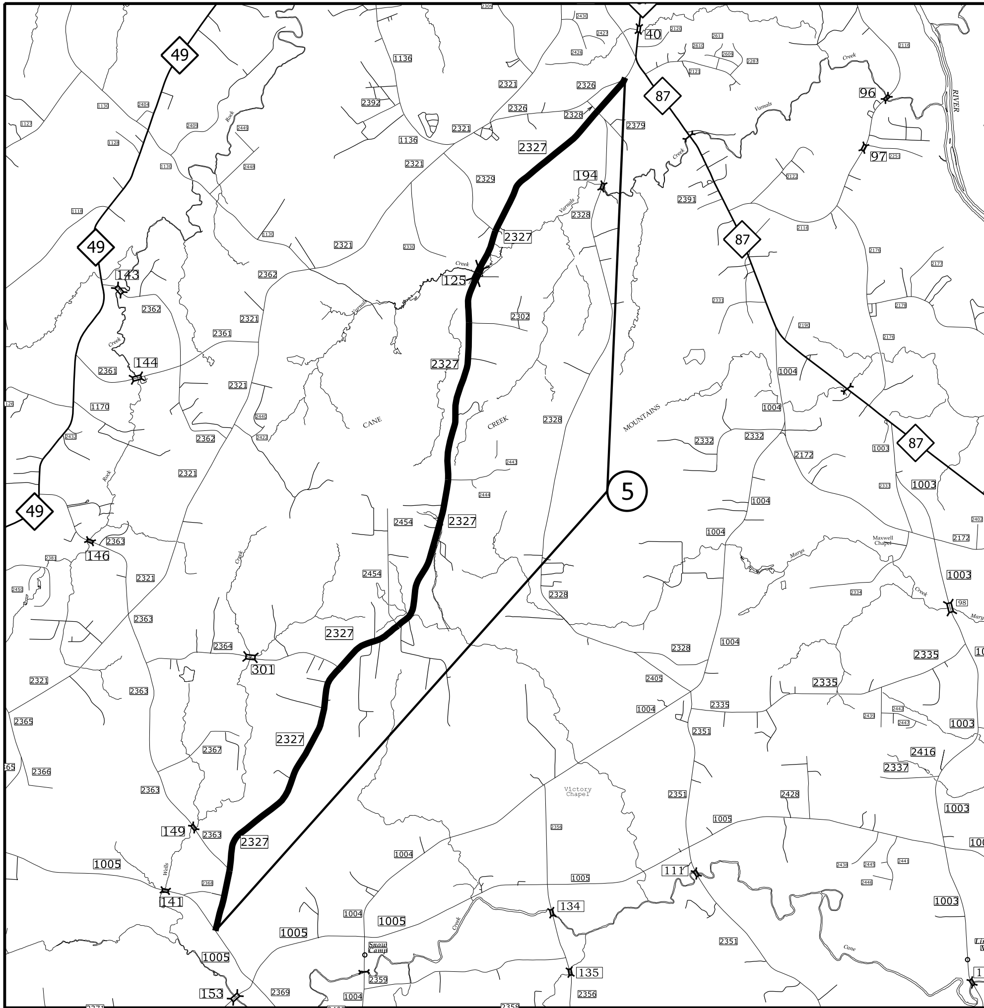
Map 5 SR 2327 Bass Mountain Rd Incidental Mill at Bridge #125 Bridge Approaches Mill and Fill 1-1/2" on Bridge #125
