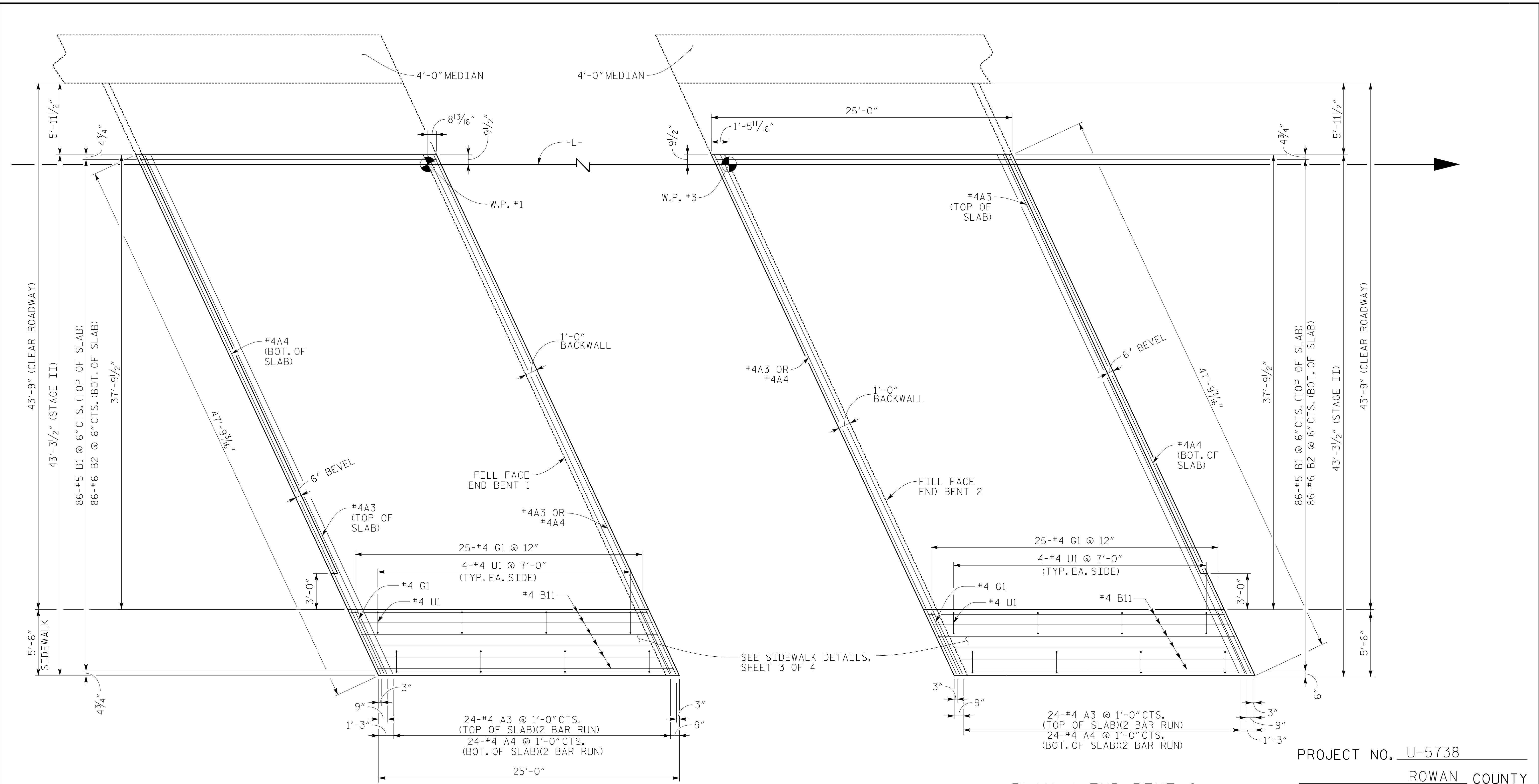
PLAN @ END BENT 1 STAGE II
