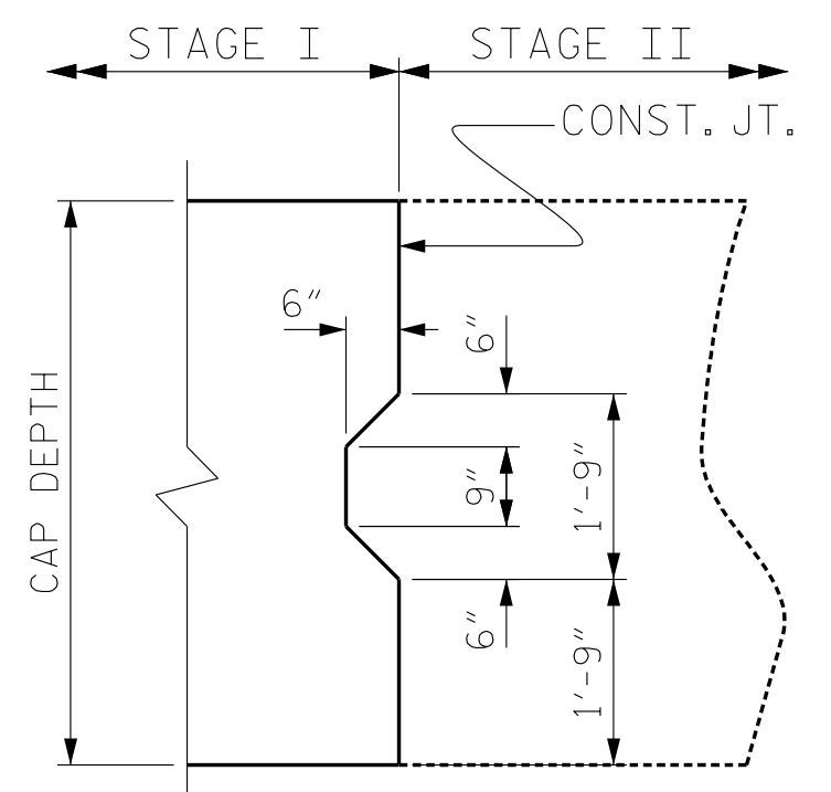
SHEAR KEY DETAIL
