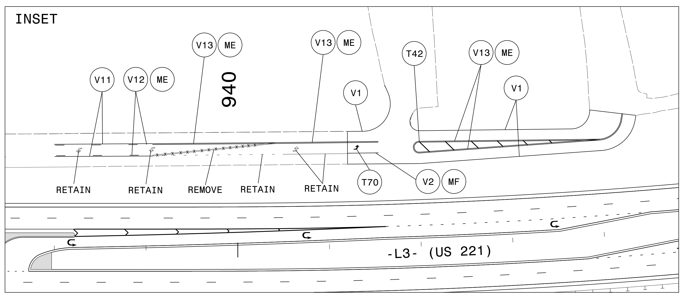
PAVEMENT MARKING DETAIL
