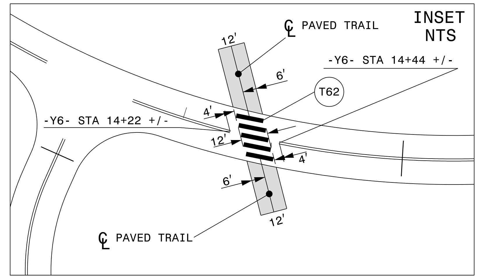
PAVEMENT MARKING DETAIL
