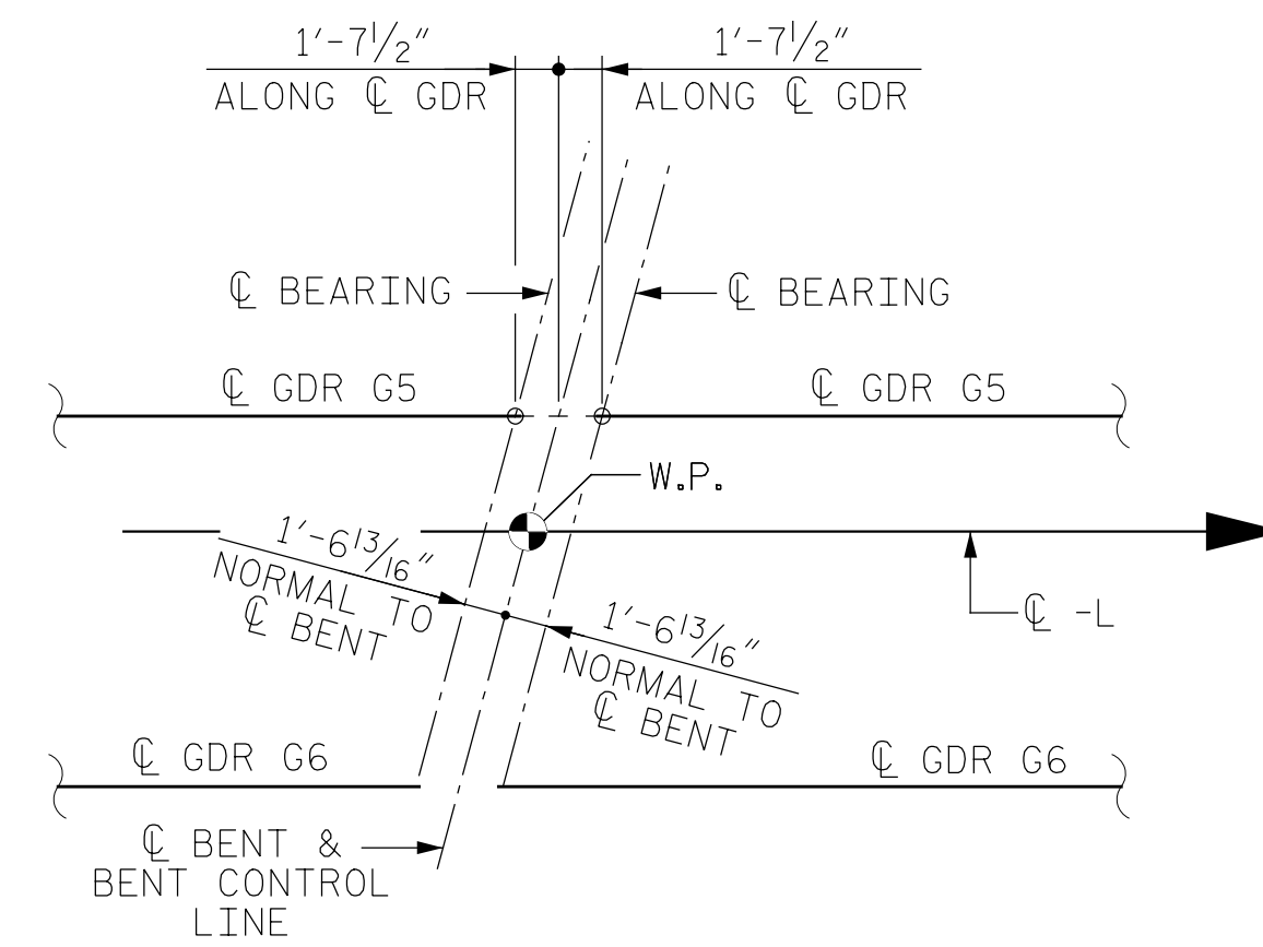
DETAIL C (TYPICAL AT BENT 3 & 5)
