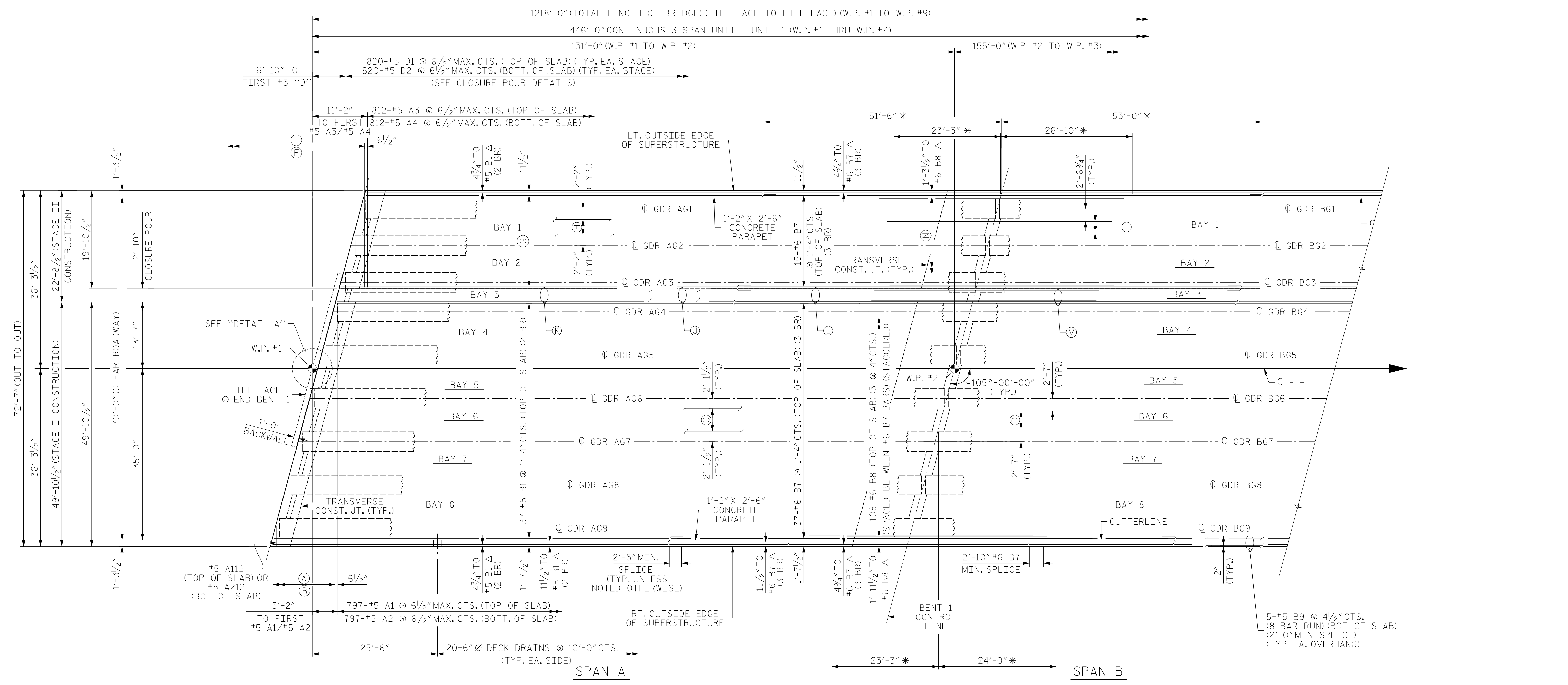
PLAN OF SPAN A AND PARTIAL PLAN OF SPAN B
