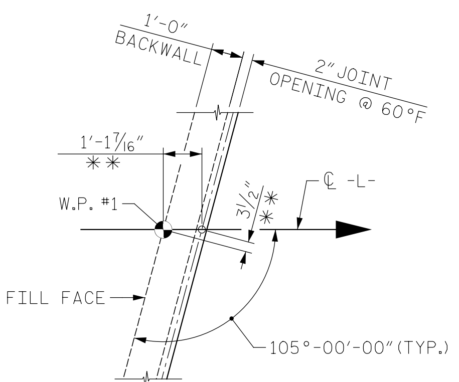
DETAIL A ** W.P. TO CL JOINT
