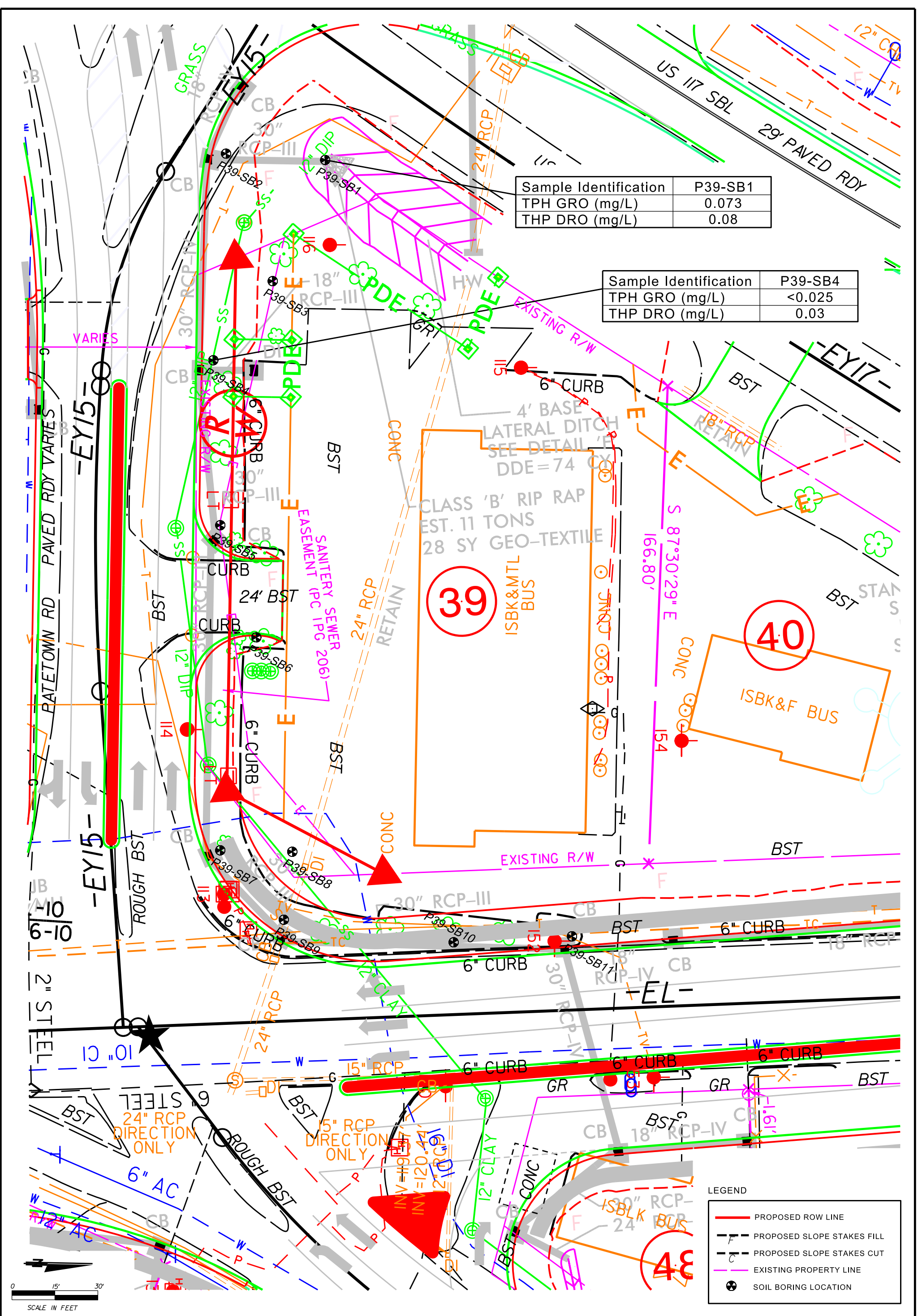
FIGURE 4 PARCEL 39 ONSITE UVF HYDROCARBON ANALYSIS RESULTS - GROUNDWATER 6/15/17
