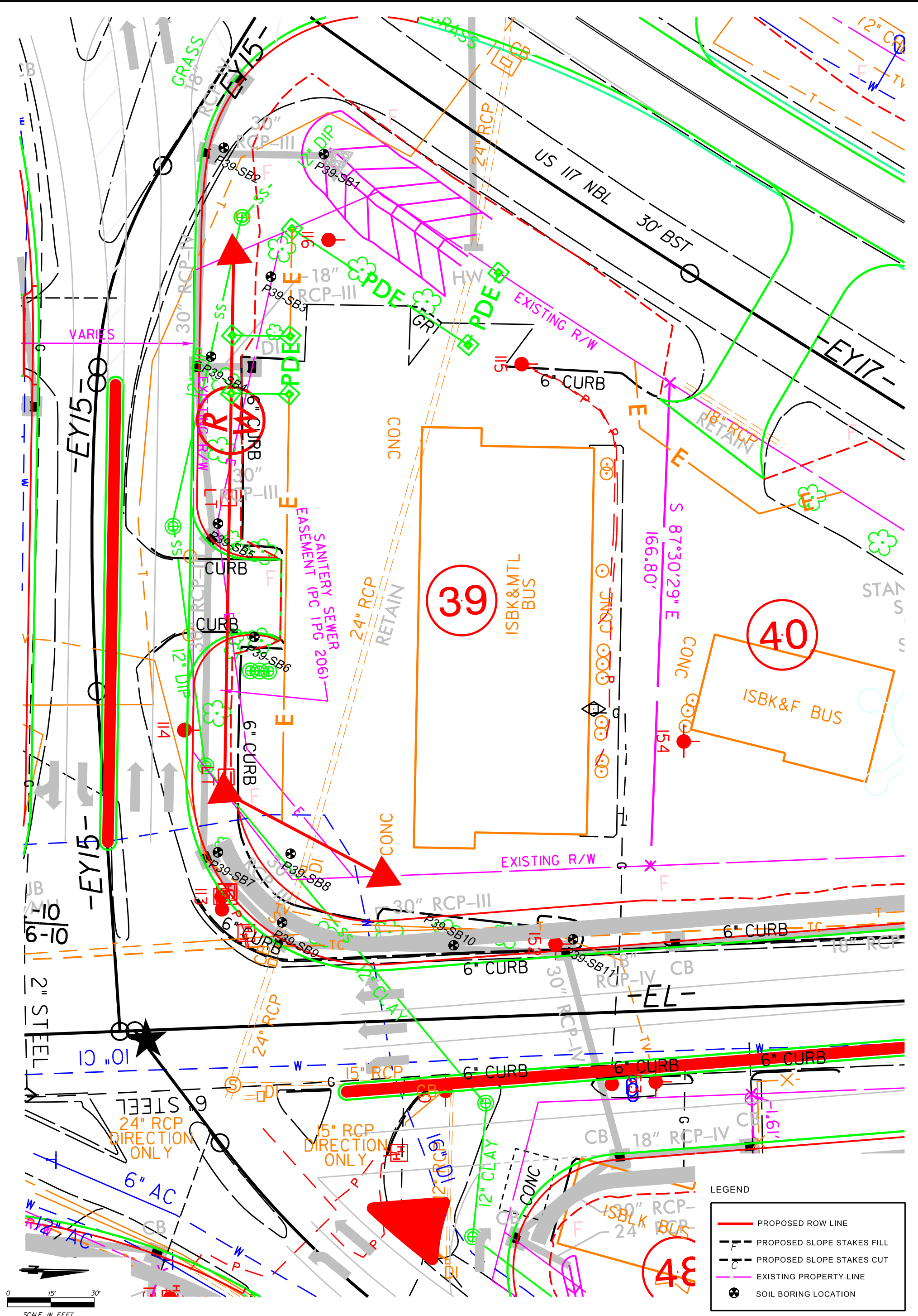
FIGURE 2 PARCEL 39 SITE MAP WITH SOIL BORING LOCATIONS
