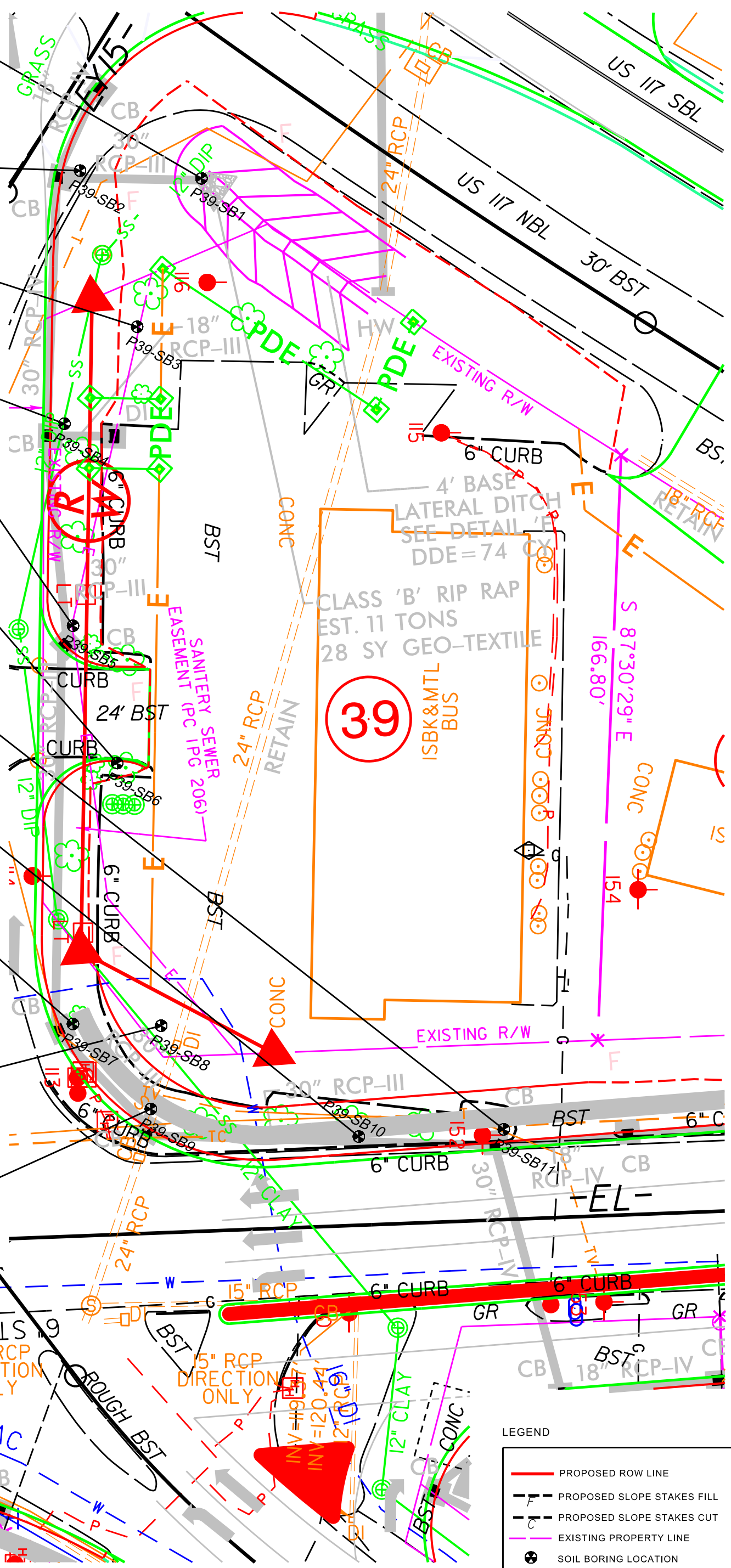
FIGURE 3 PARCEL 39 ONSITE UVF HYDROCARBON ANALYSIS RESULTS - SOIL 6/15/17
