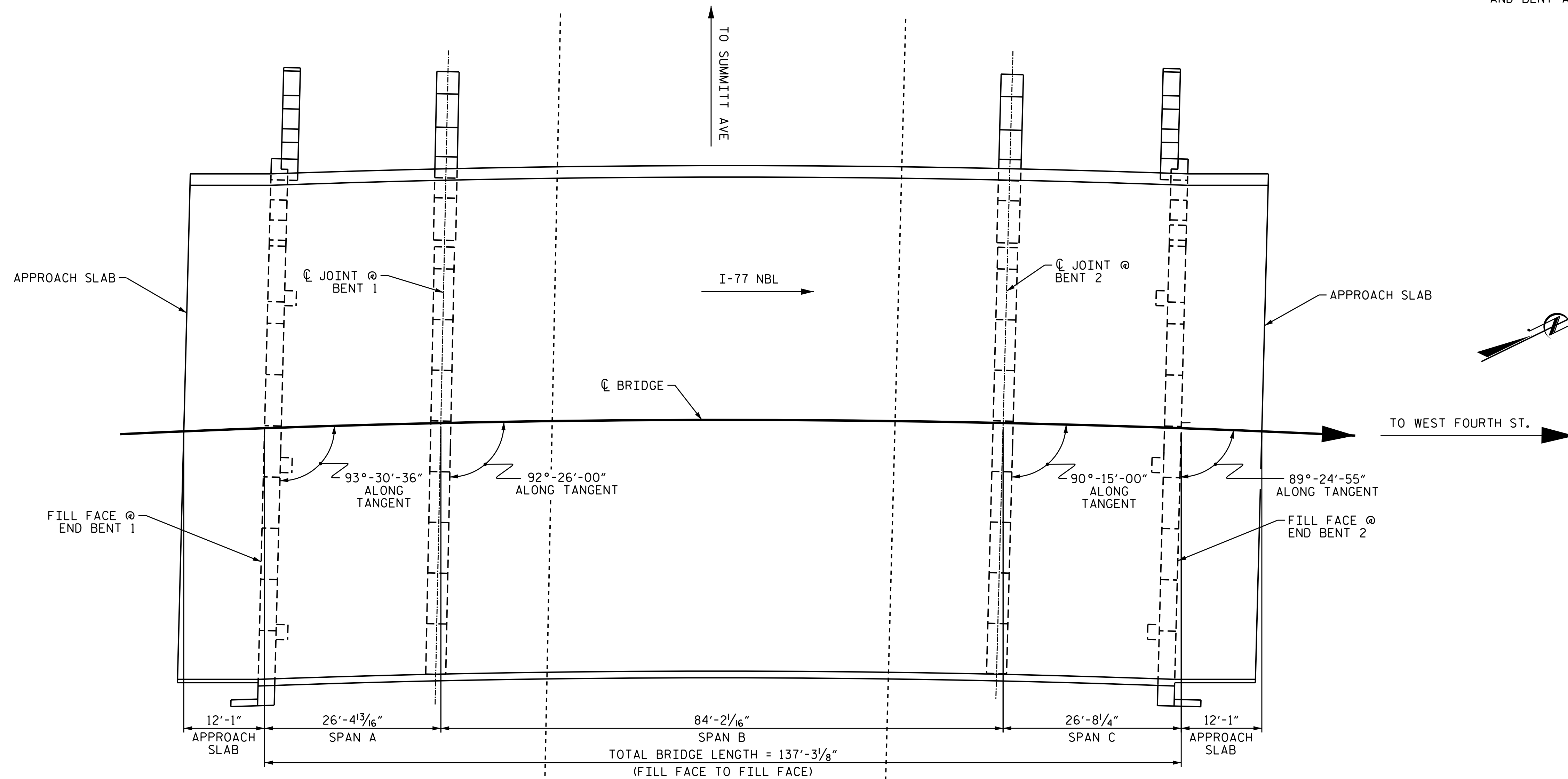
PLAN FOUNDATIONS NOT SHOWN FOR CLARITY
