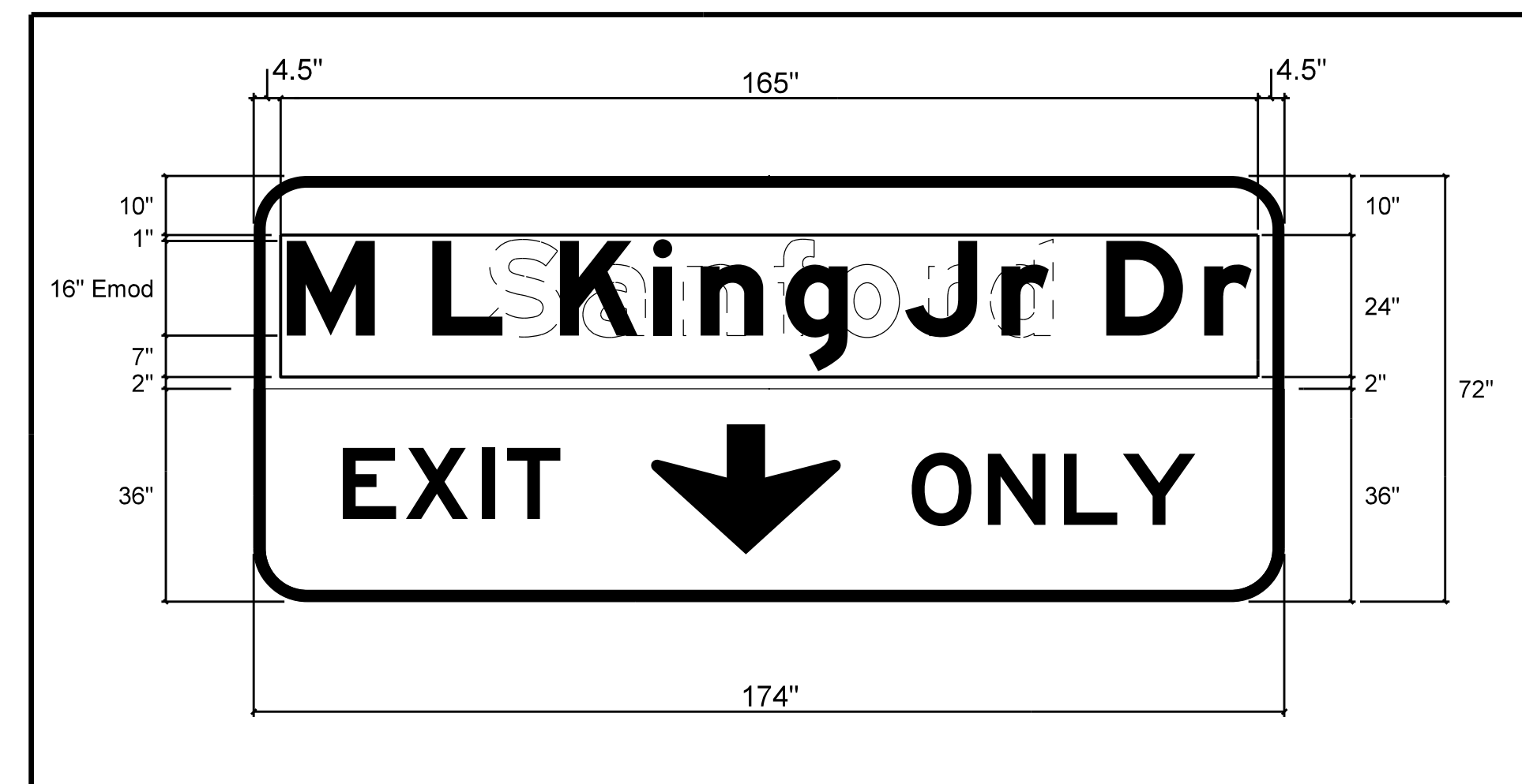
Overlay Placement Detail Overlay Panel #702 (165" x 24")
