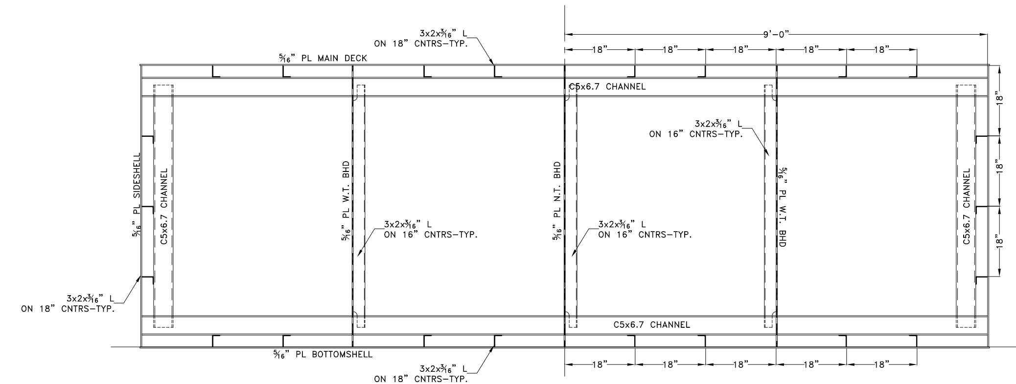
XVERSE STRUCTURAL DETAILS @ FR 5 SHOWN LKG FWD DETAILS @ FR 2, 4, 6 & 8 SIMILAR 6 & 8 OPP. HAND
