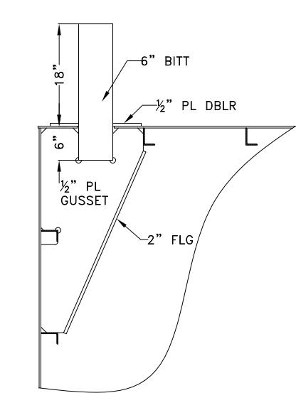
TYPICAL XVERSE SECTION IWO PIPE BITS
