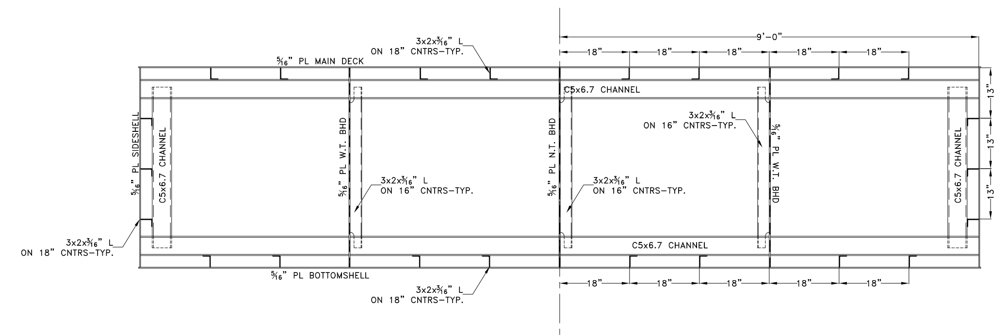
XVERSE STRUCTURAL DETAILS @ FR 1 SHOWN LKG FWD DETAILS @ FR 9 SIM. OPP. HAND
