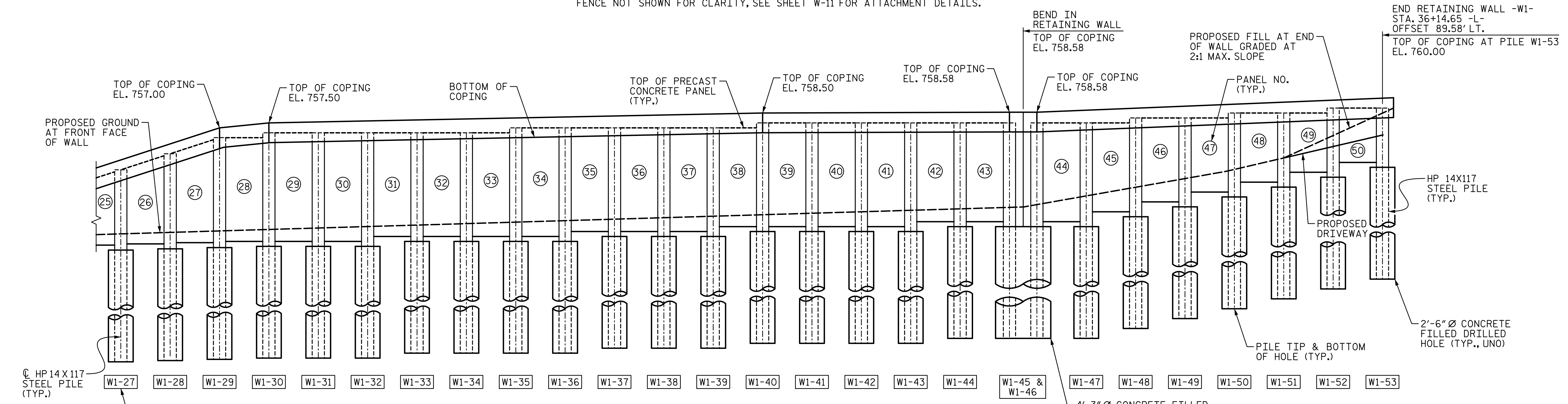
RETAINING WALL -W1- ELEVATION BOTTOM OF CONCRETE FILLED DRILLED HOLE NOT TO SCALE. FENCE NOT SHOWN FOR CLARITY, SEE SHEET W-11 FOR ATTACHMENT DETAILS.
