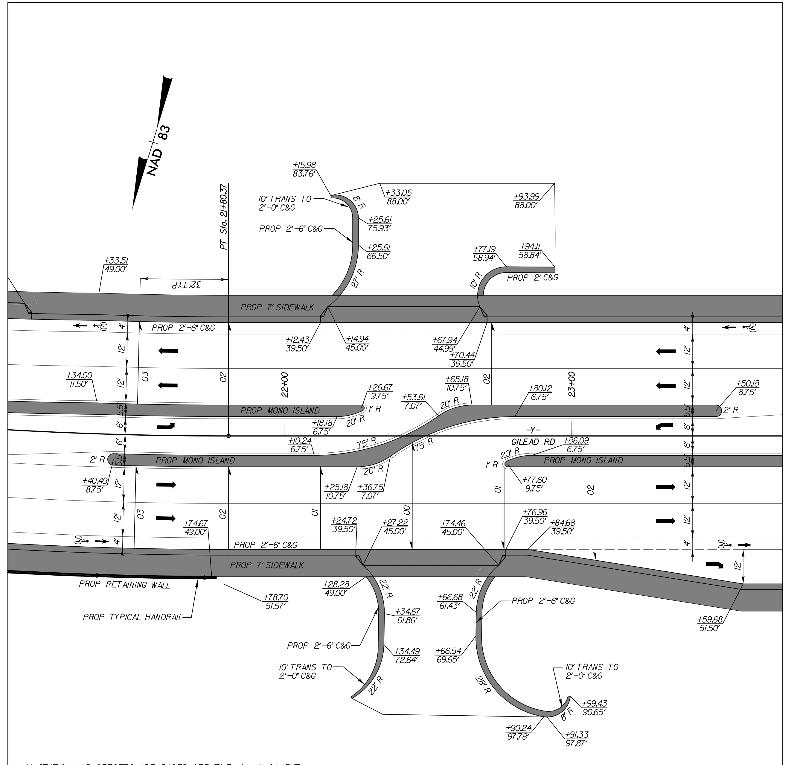
0 20 40 SEE SHEET 6 FOR FULL PLAN VIEW SCALE : 1" = 20' -Y- GILEAD RD
