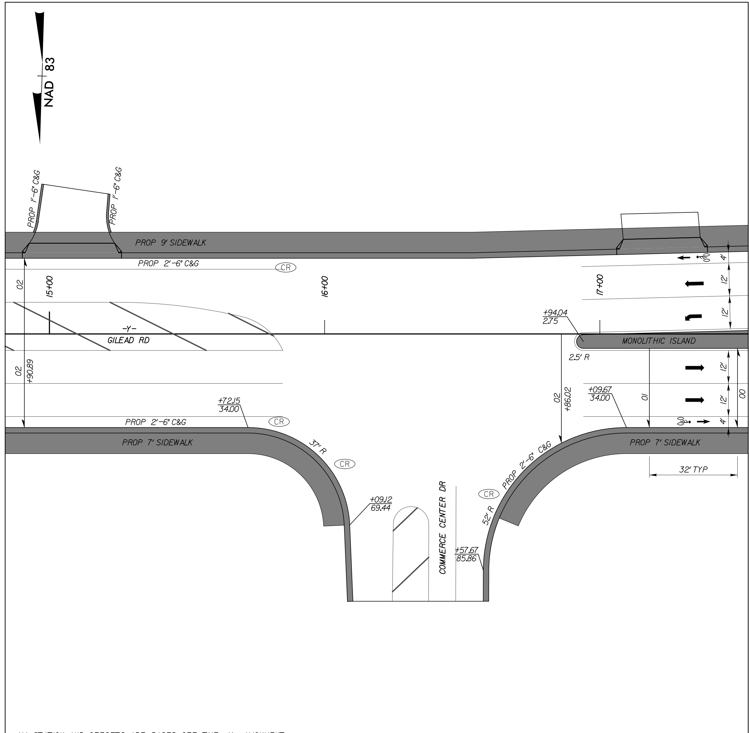
0 20 40 SEE SHEET 8 FOR FULL PLAN VIEW SCALE : 1" = 20' -Y- GILEAD RD, COMMERCE CENTER DR
