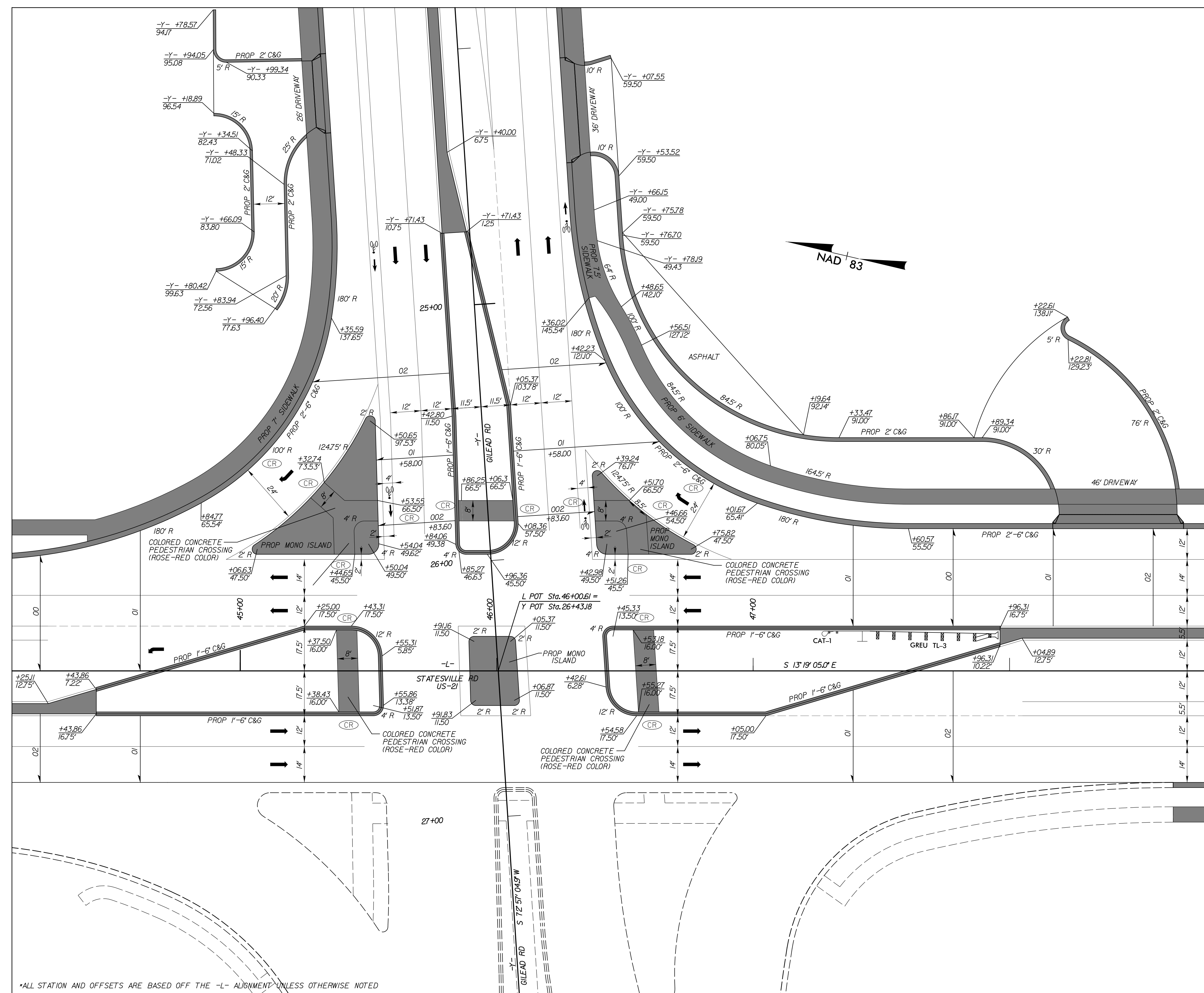
INTERSECTION DETAIL - A
