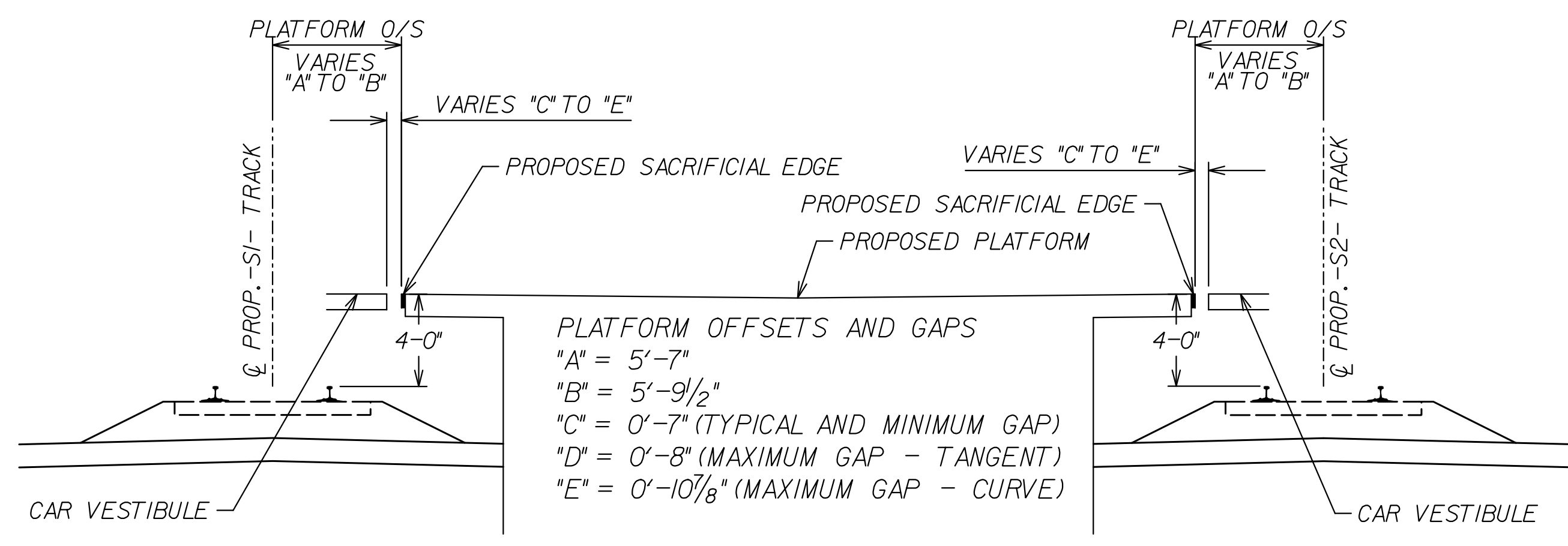
PLATFORM OFFSET DETAIL NOT TO SCALE
