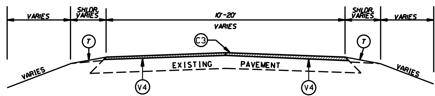
TYPICAL SECTION NO. 39
