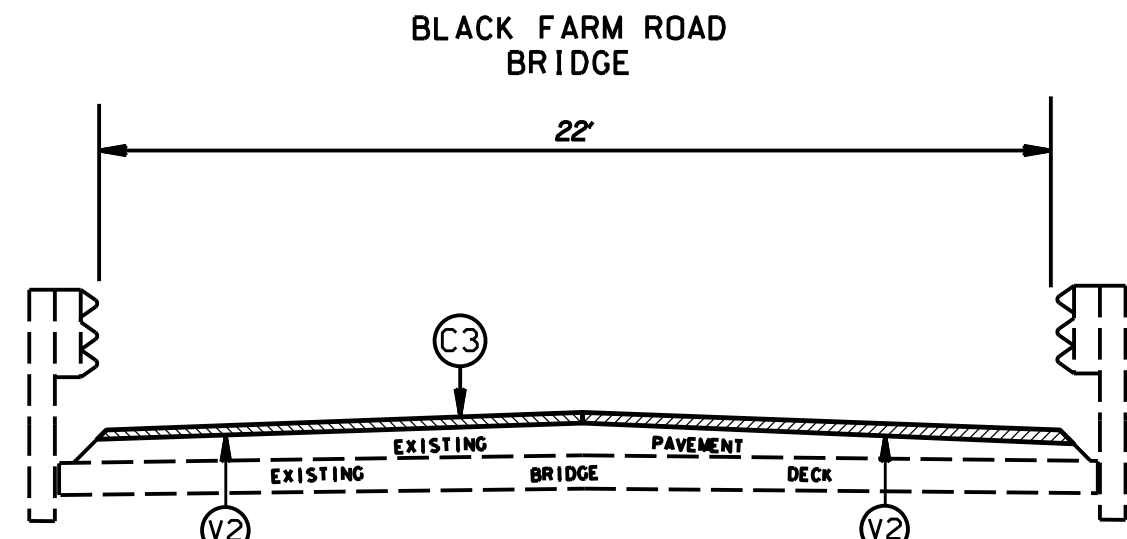
TYPICAL SECTION NO. 38
