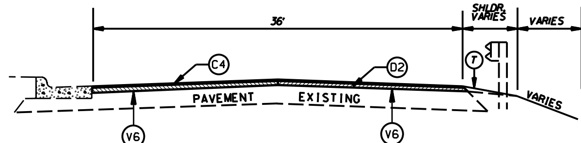
TYPICAL SECTION NO. 23
