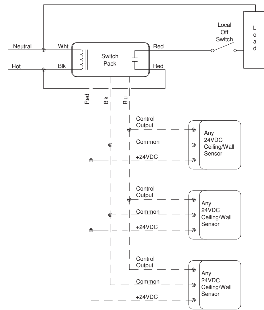
1 E1.1 TYPICAL MULTIPLE SENSOR LIGHTING CONTROL DETAIL 1/2" = 1'-0"
