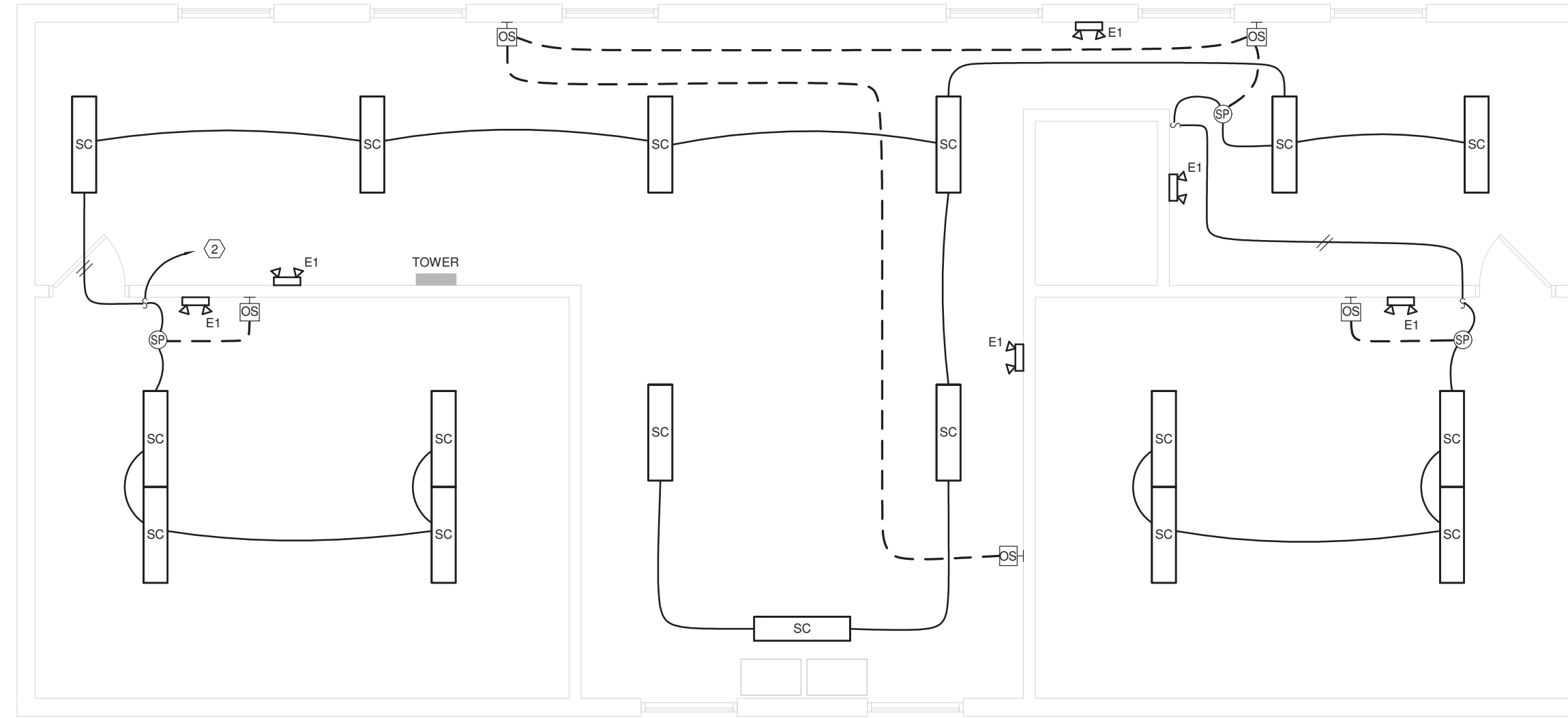
TOWER PLAN
