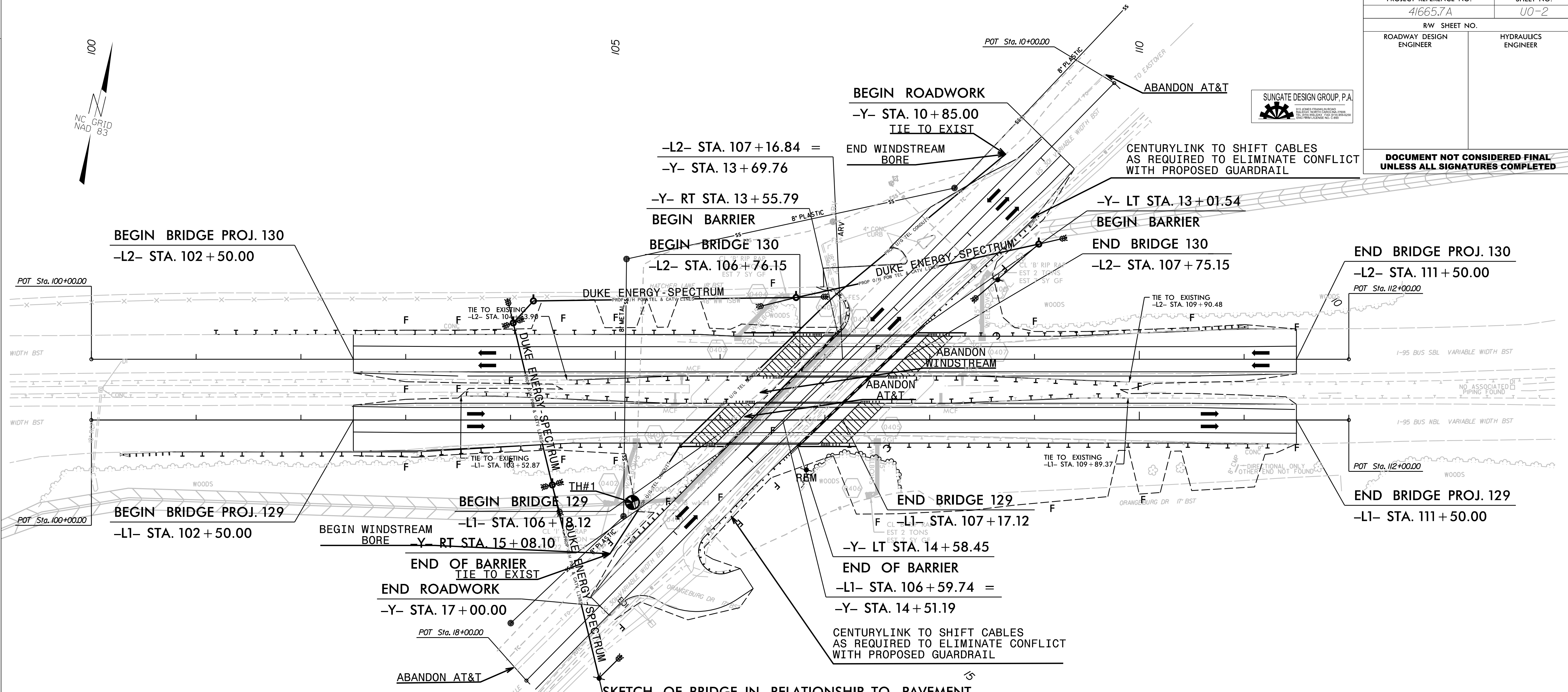
SKETCH OF BRIDGE IN RELATIONSHIP TO PAVEMENT
