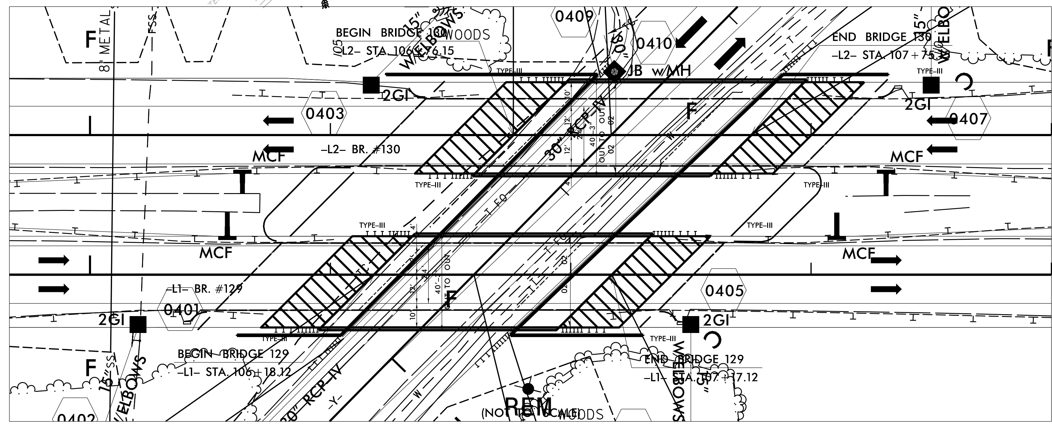
SKETCH OF BRIDGE IN RELATIONSHIP TO PAVEMENT
