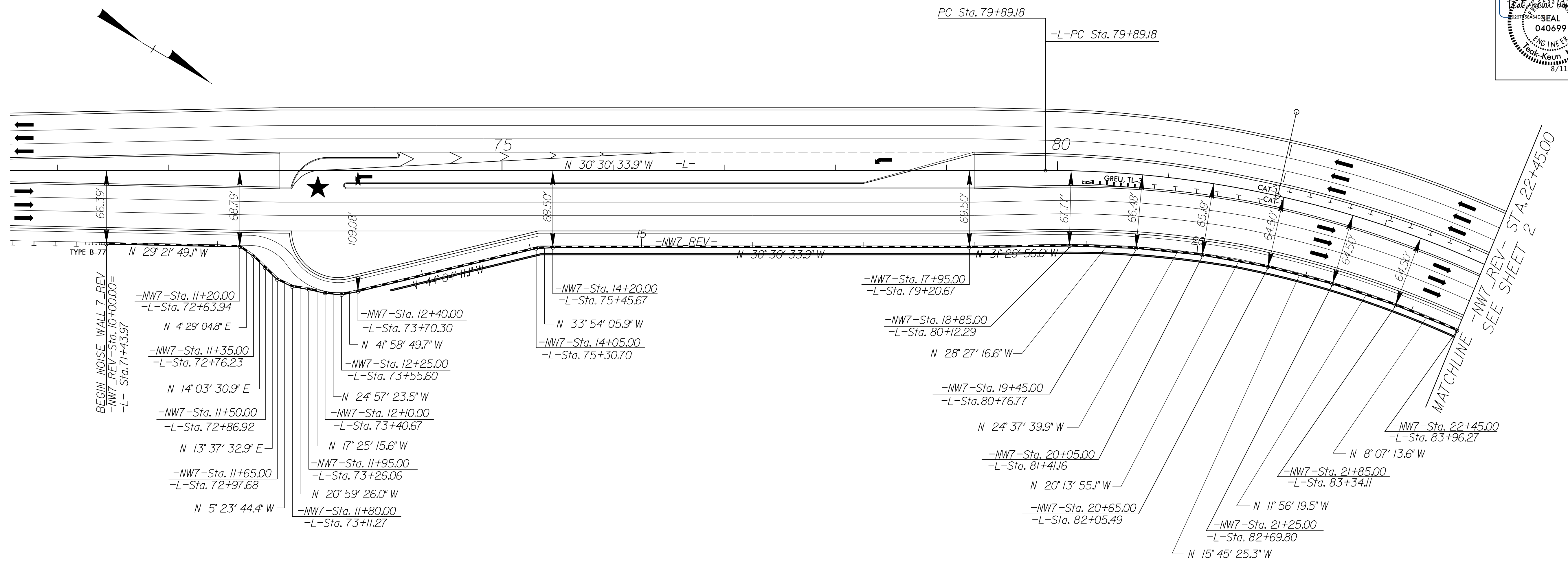
NOISE WALL 7_REV DESIGN DATA
