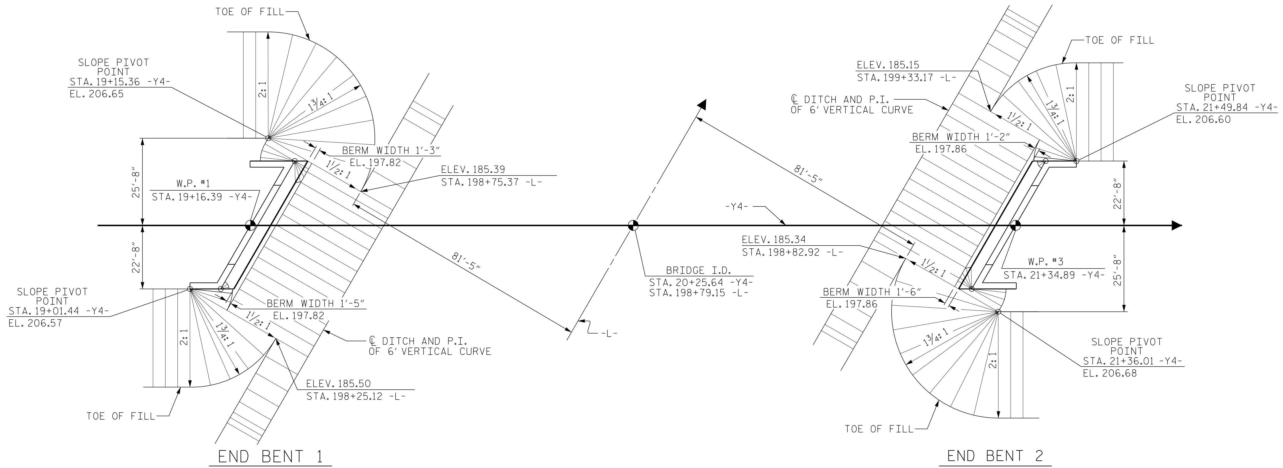
PLAN - GRADING
