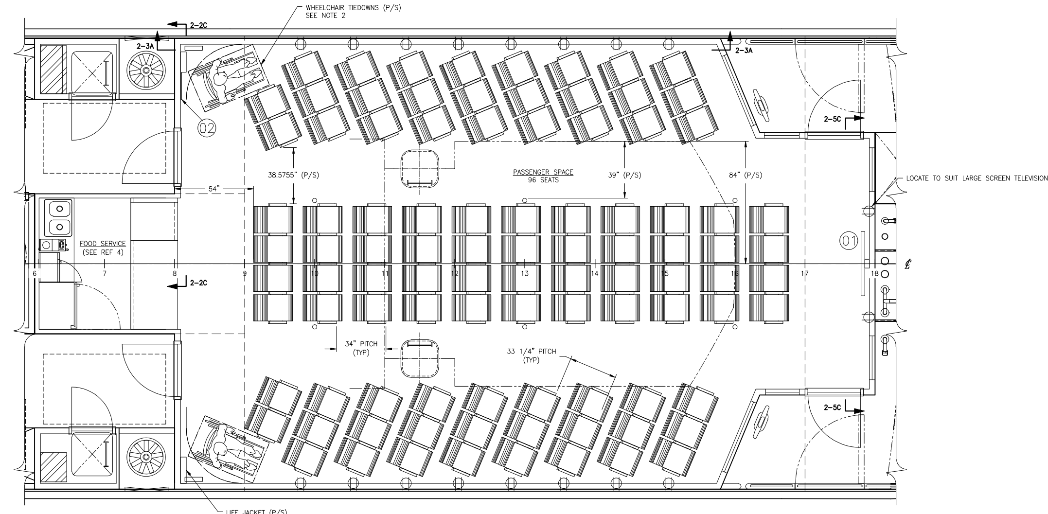
PLAN 1-4A MAIN DECK SCALE: 3/8"=1'-0"
