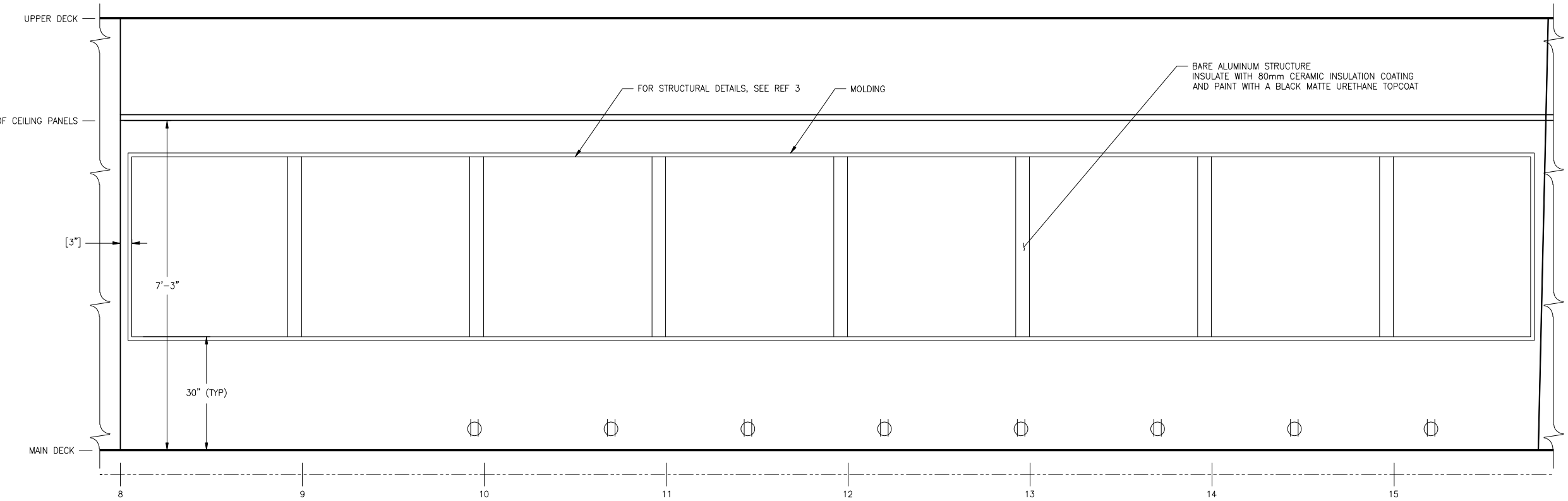
SECTION 2-2C FRAME 8 LOOKING AFT PORT SIDE SHOWN, STBD SIMILAR SCALE: 3/4"=1'-0"
