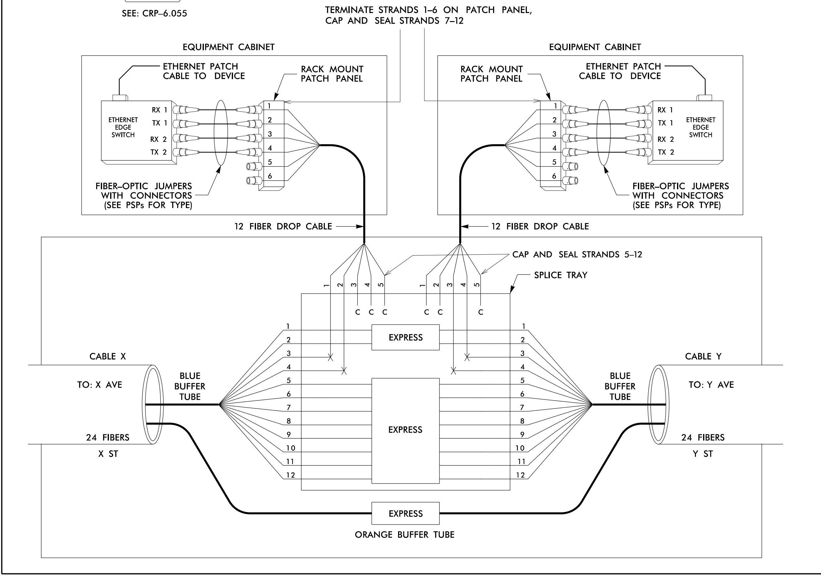
SPLICE ENCLOSURE NO. S20-1
