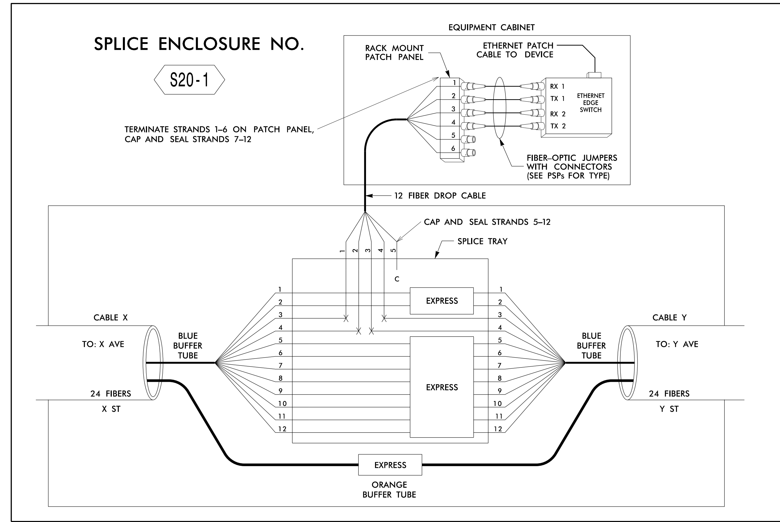
SPLICE ENCLOSURE NO. S20-1
