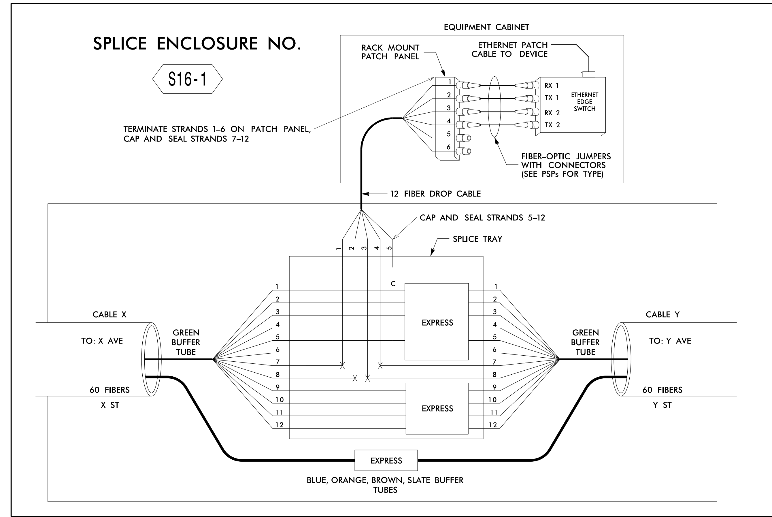
SPLICE ENCLOSURE NO. S16-1
