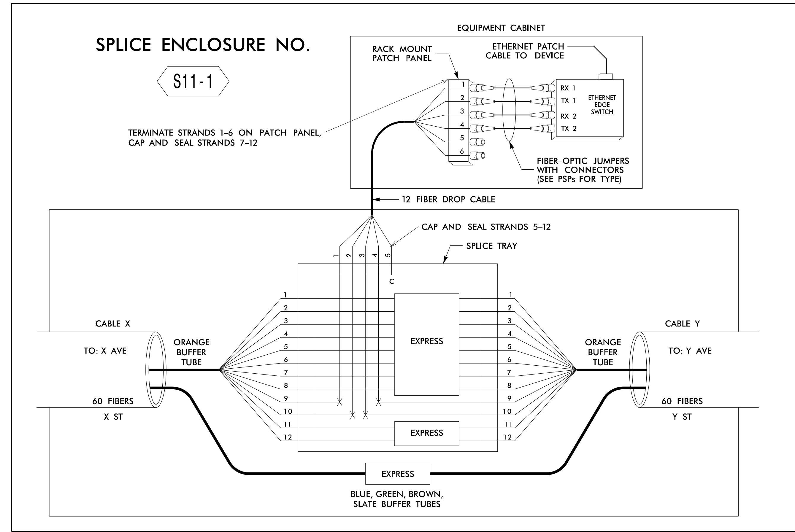
SPLICE ENCLOSURE NO. S11-1
