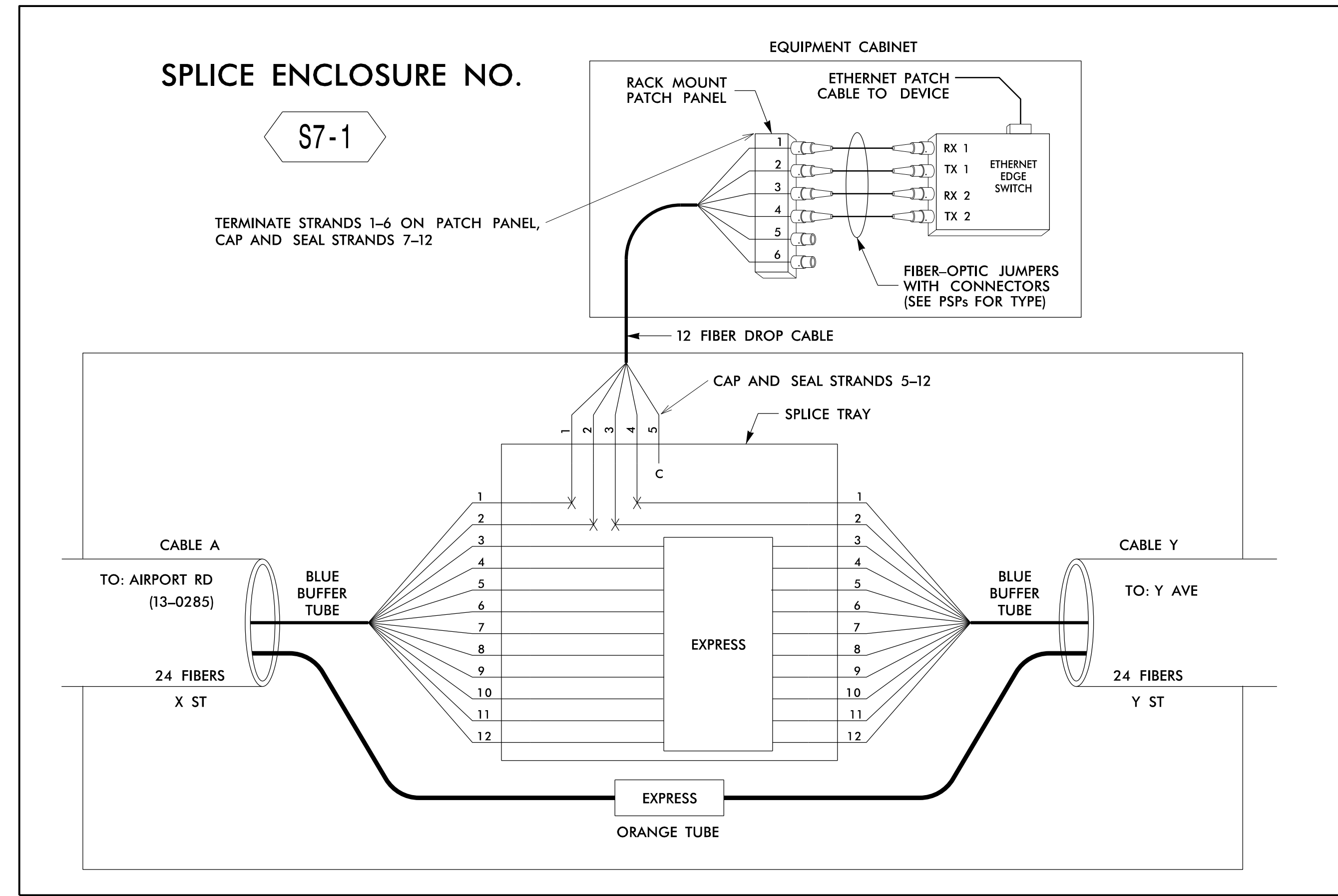
SPLICE ENCLOSURE NO. S7-1
