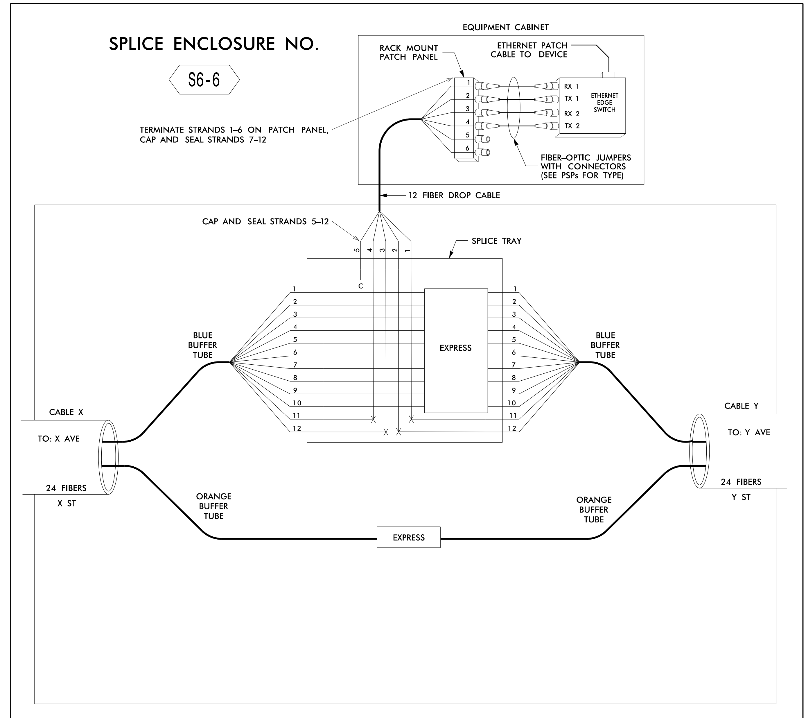
SPLICE ENCLOSURE NO. S6-6
