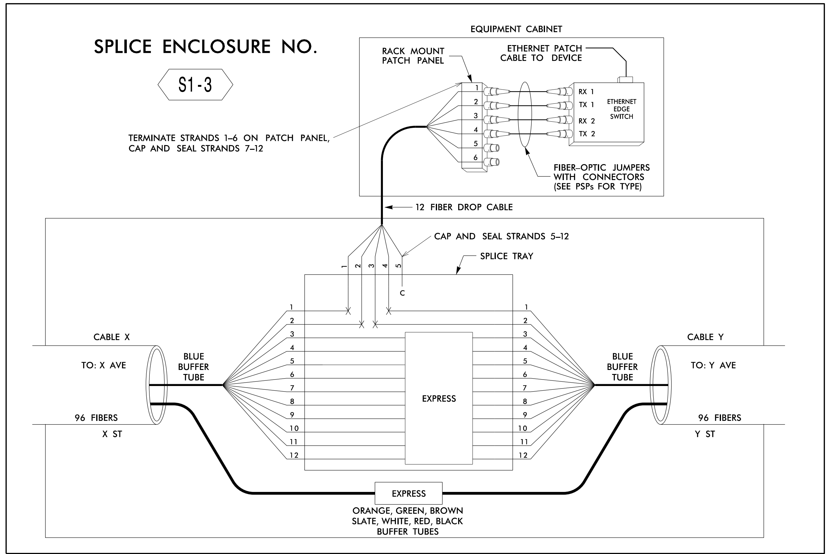
SPLICE ENCLOSURE NO. S1-3
