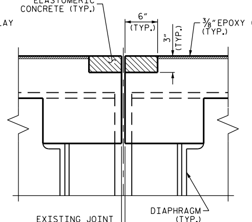
PROPOSED PRE-SAWED JOINT
