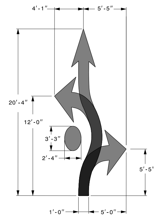
ROUNDABOUT FISH-HOOK ARROW TYPICAL
