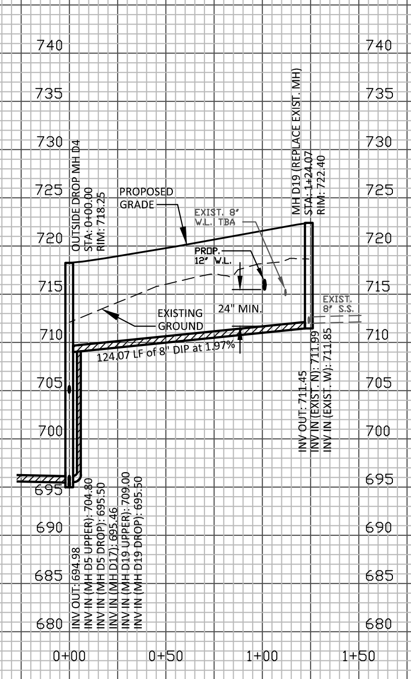
SANITARY SEWER PROFILE 8" SEWER LINE D4 - MH D4 to MH D19 STA. 0+00 to 1+24.07
