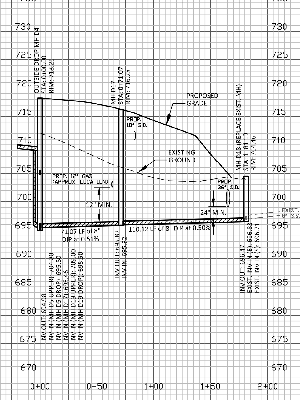
SANITARY SEWER PROFILE 8" SEWER LINE D3 - MH D4 to MH D18 STA. 0+00 to 1+81.19
