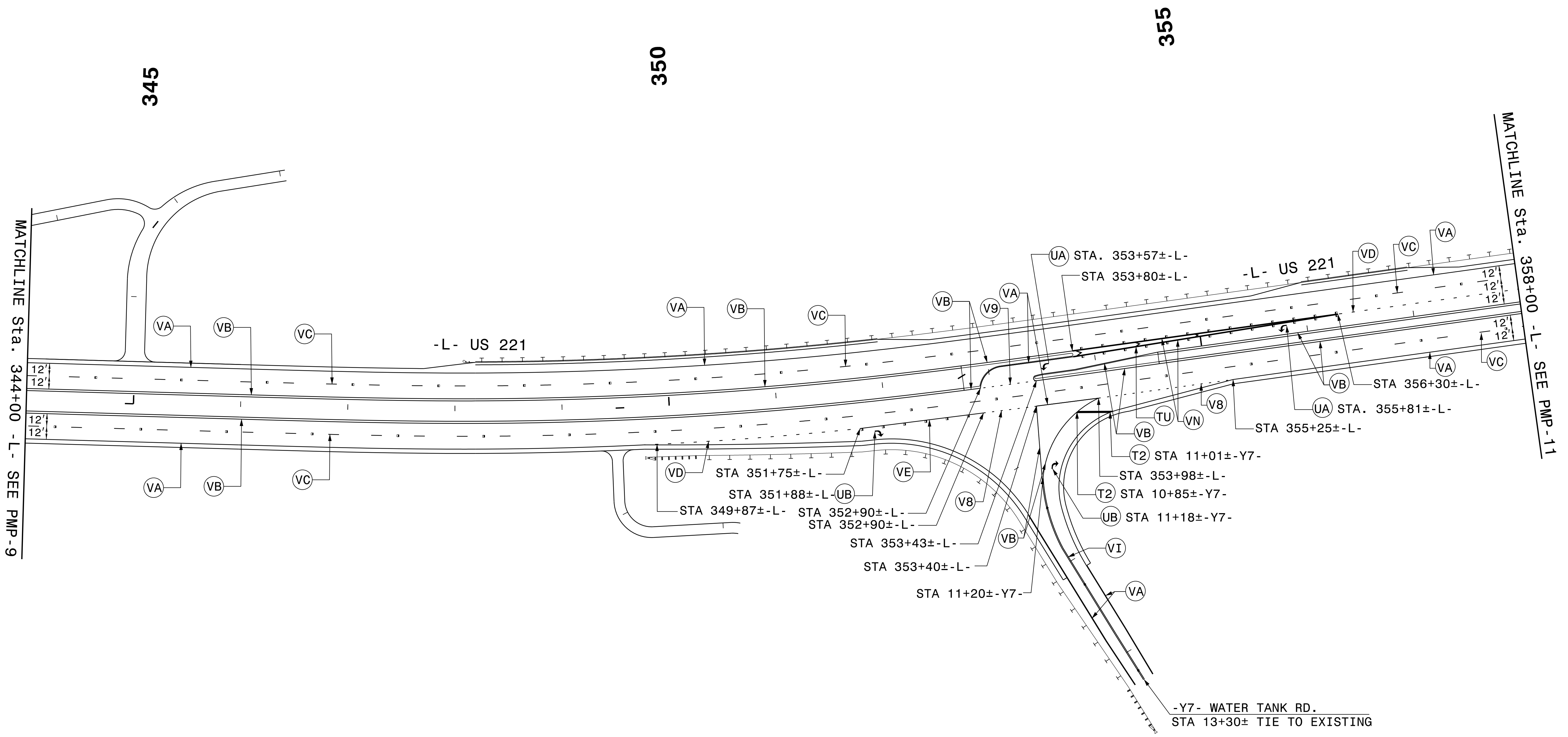
PAVEMENT MARKING DETAIL
