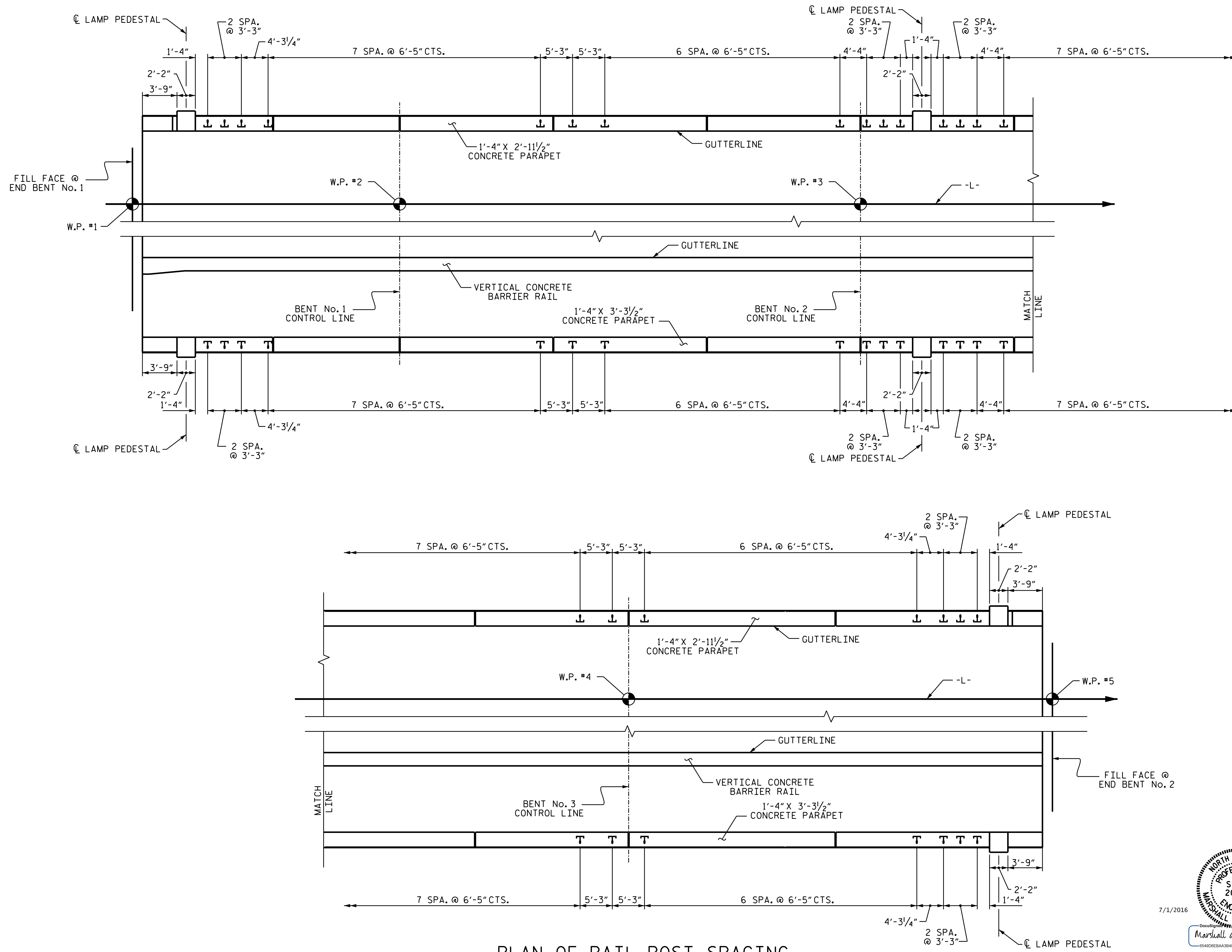
PLAN OF RAIL POST SPACING
