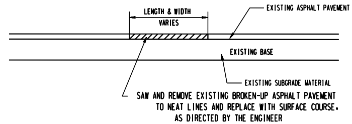
DETAIL NO. 3
