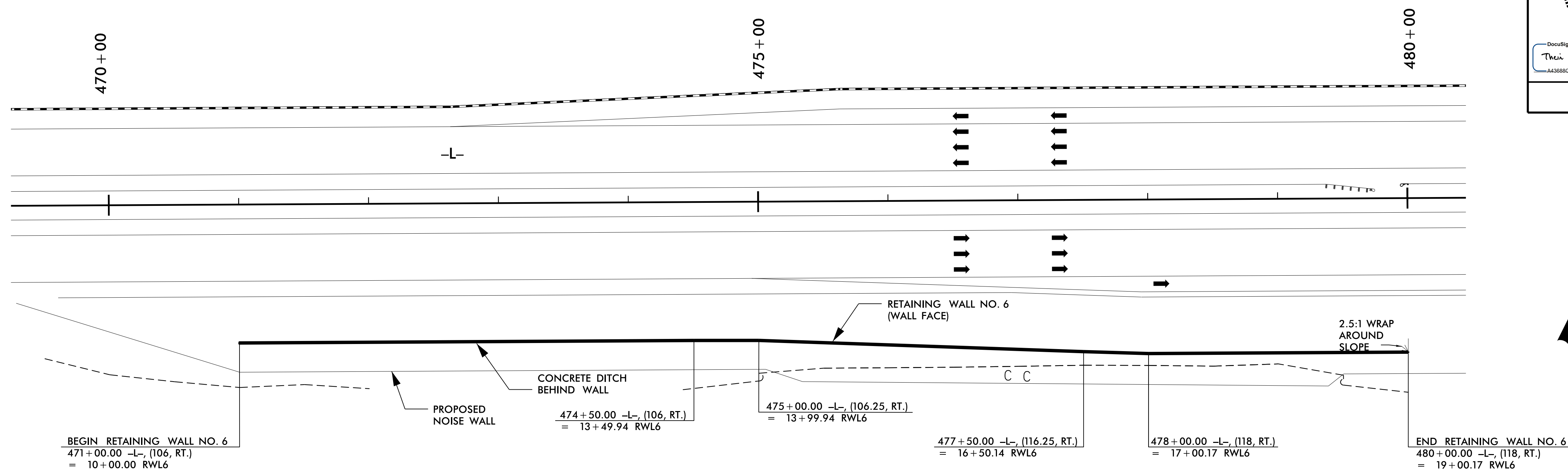
RETAINING WALL NO. 6 PLAN VIEW
