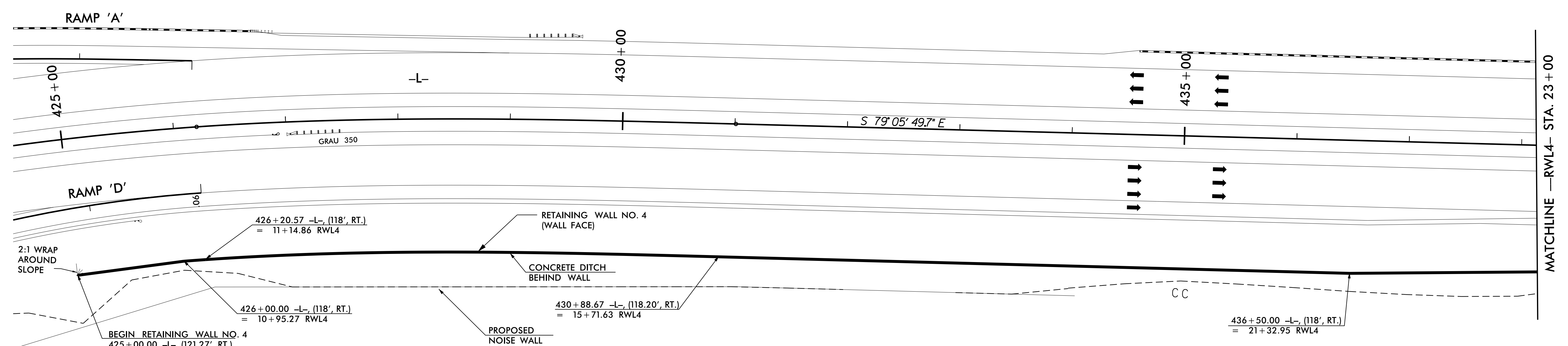
RETAINING WALL NO. 4 PLAN VIEW (PART 1)
