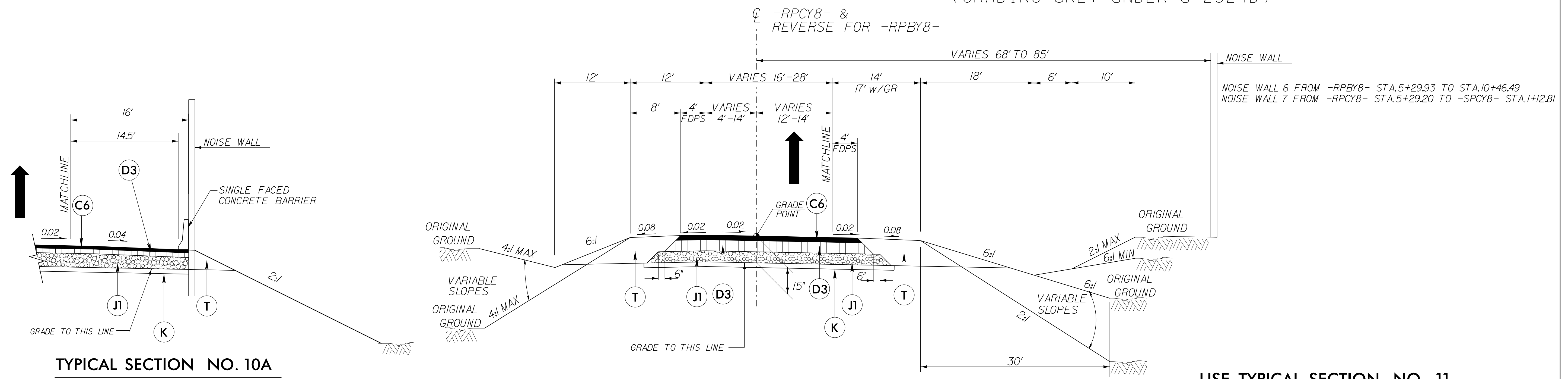
TYPICAL SECTION NO. 11
