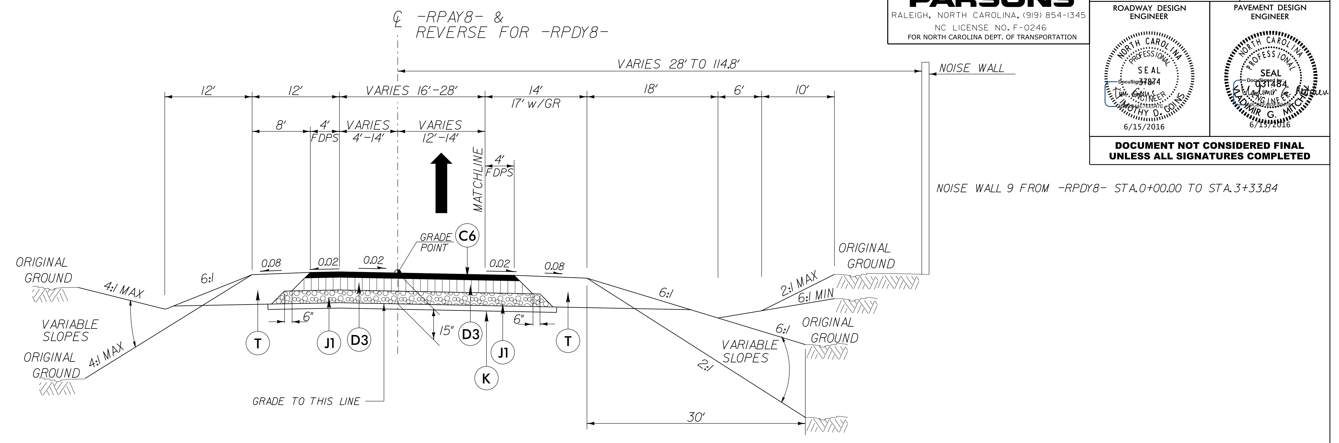
TYPICAL SECTION NO. 10
