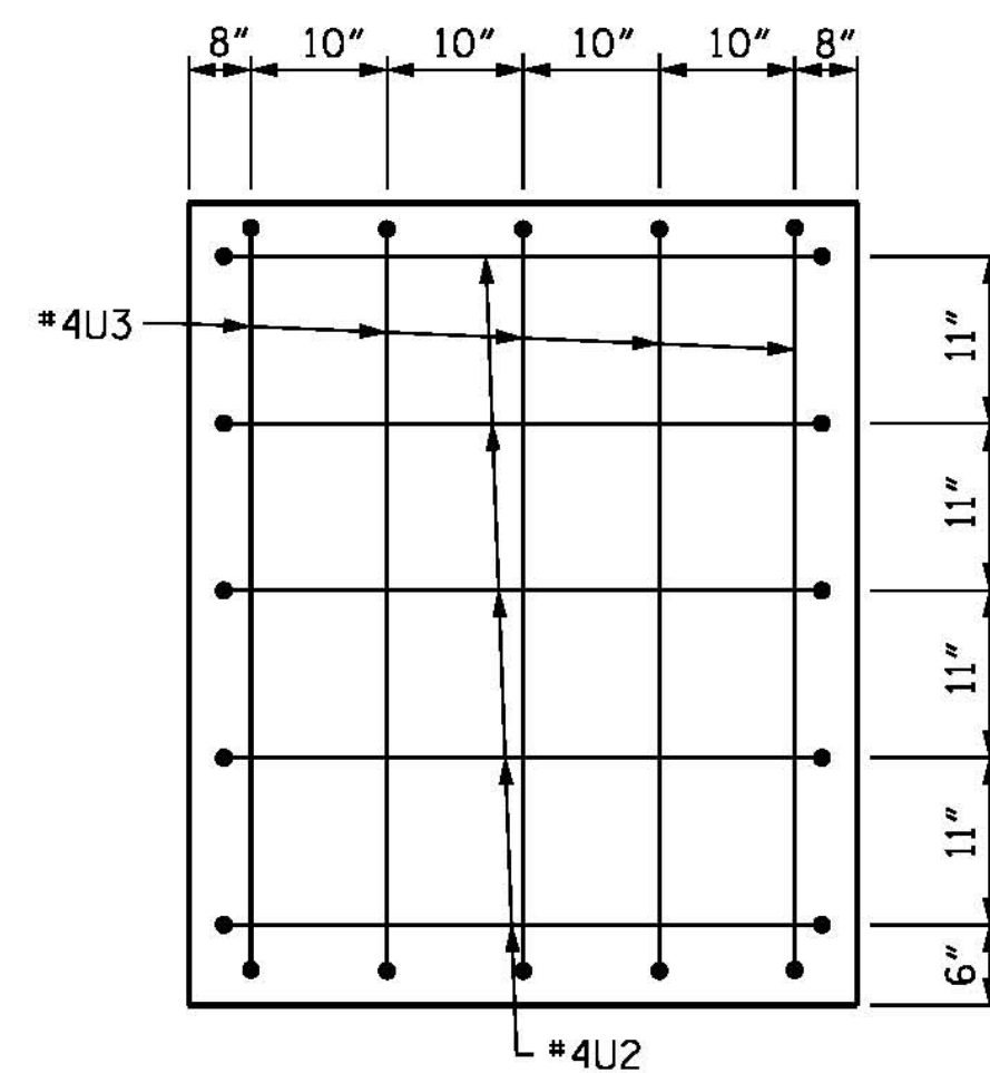
VIEW X-X
