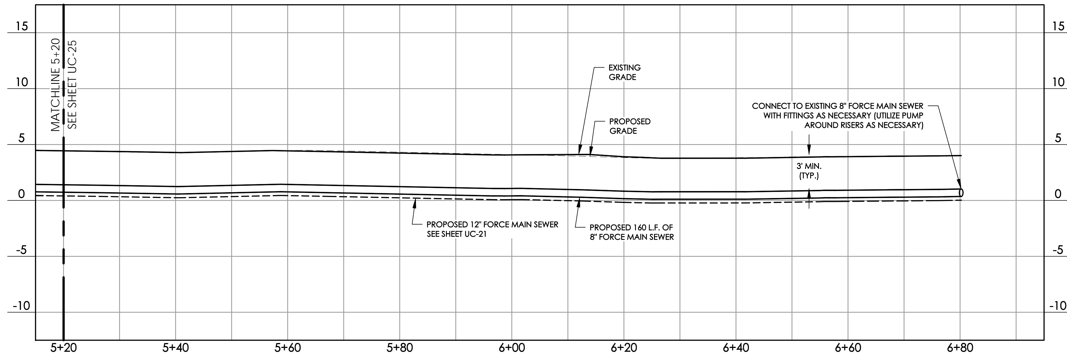
ISLAND 8" FORCE MAIN SEWER STA. 5+20 TO 6+80
