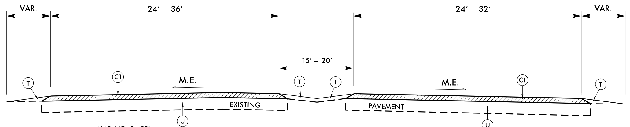
TYPICAL SECTION NO. 3
