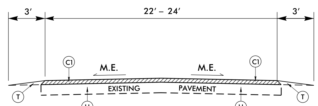
TYPICAL SECTION NO. 4
