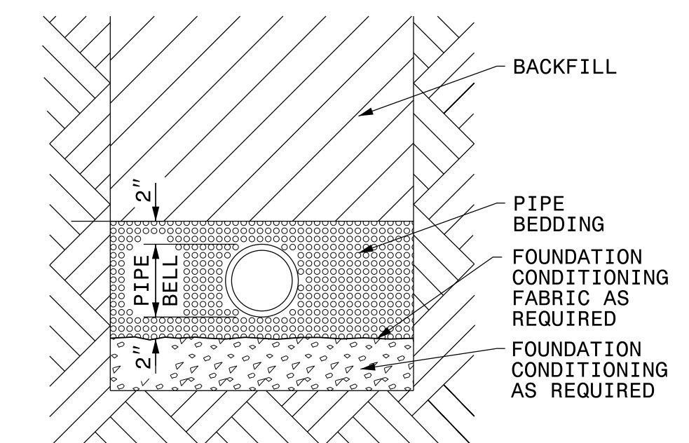
TRENCH DETAIL
