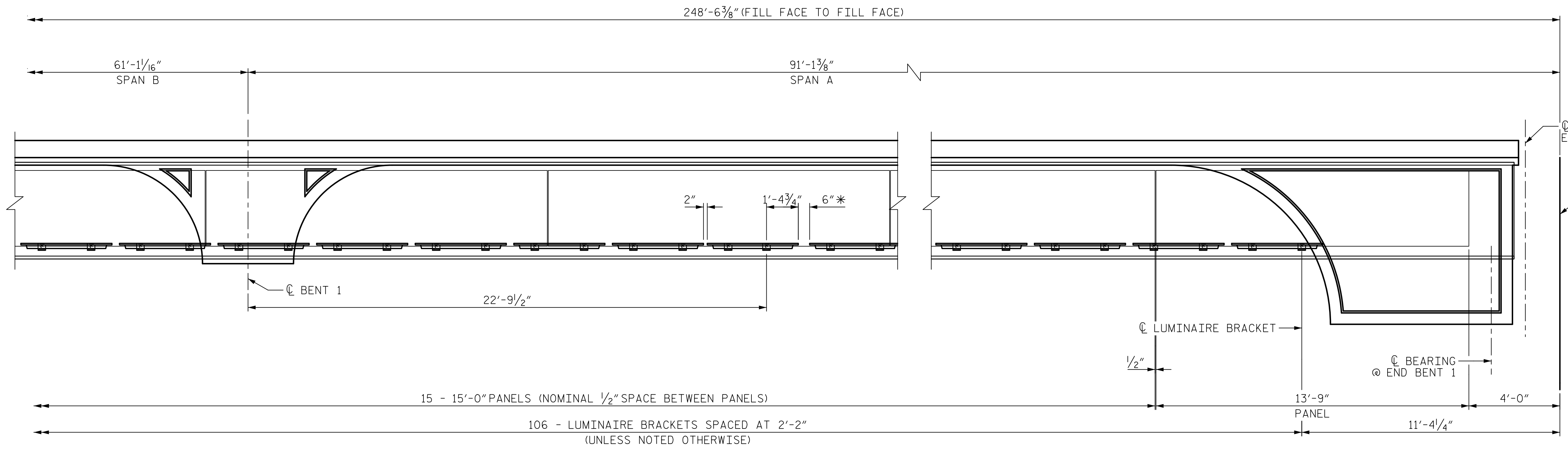
ELEVATION ALONG CL GIRDER 1
