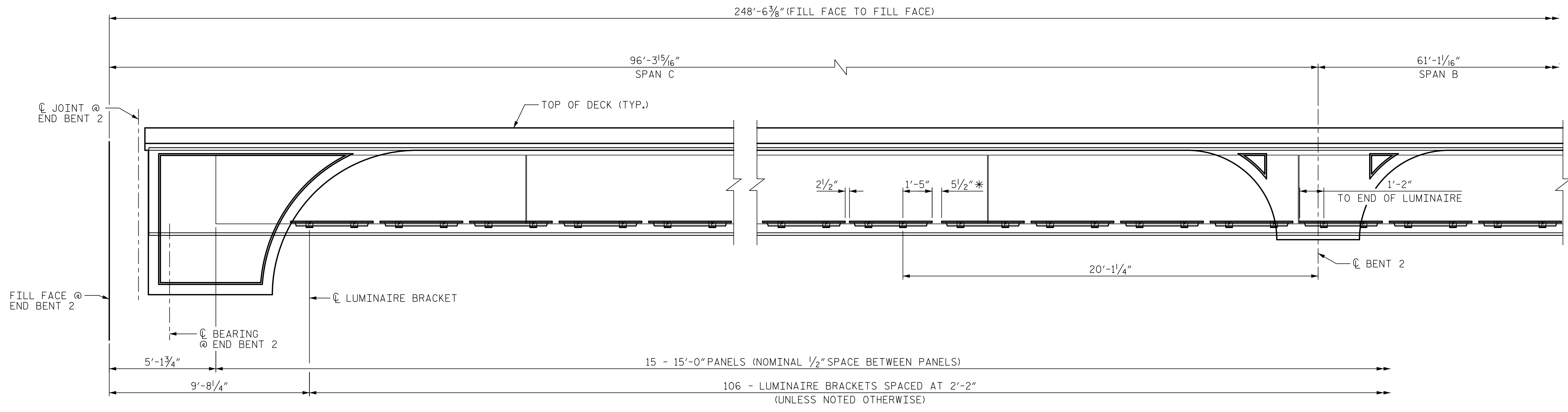
ELEVATION ALONG CL GIRDER 1
