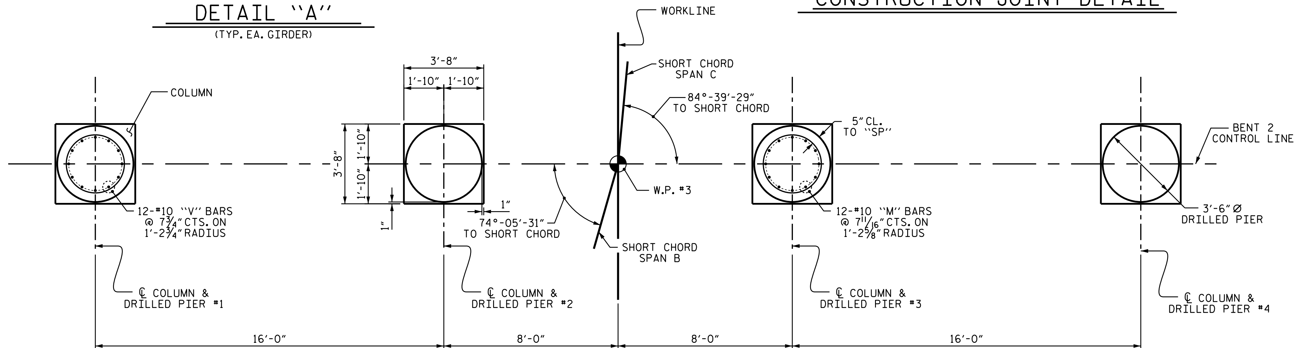
PLAN OF COLUMNS & DRILLED PIERS REINFORCING STEEL AND DIMENSIONS ARE TYPICAL FOR EACH COLUMN AND DRILLED PIER
