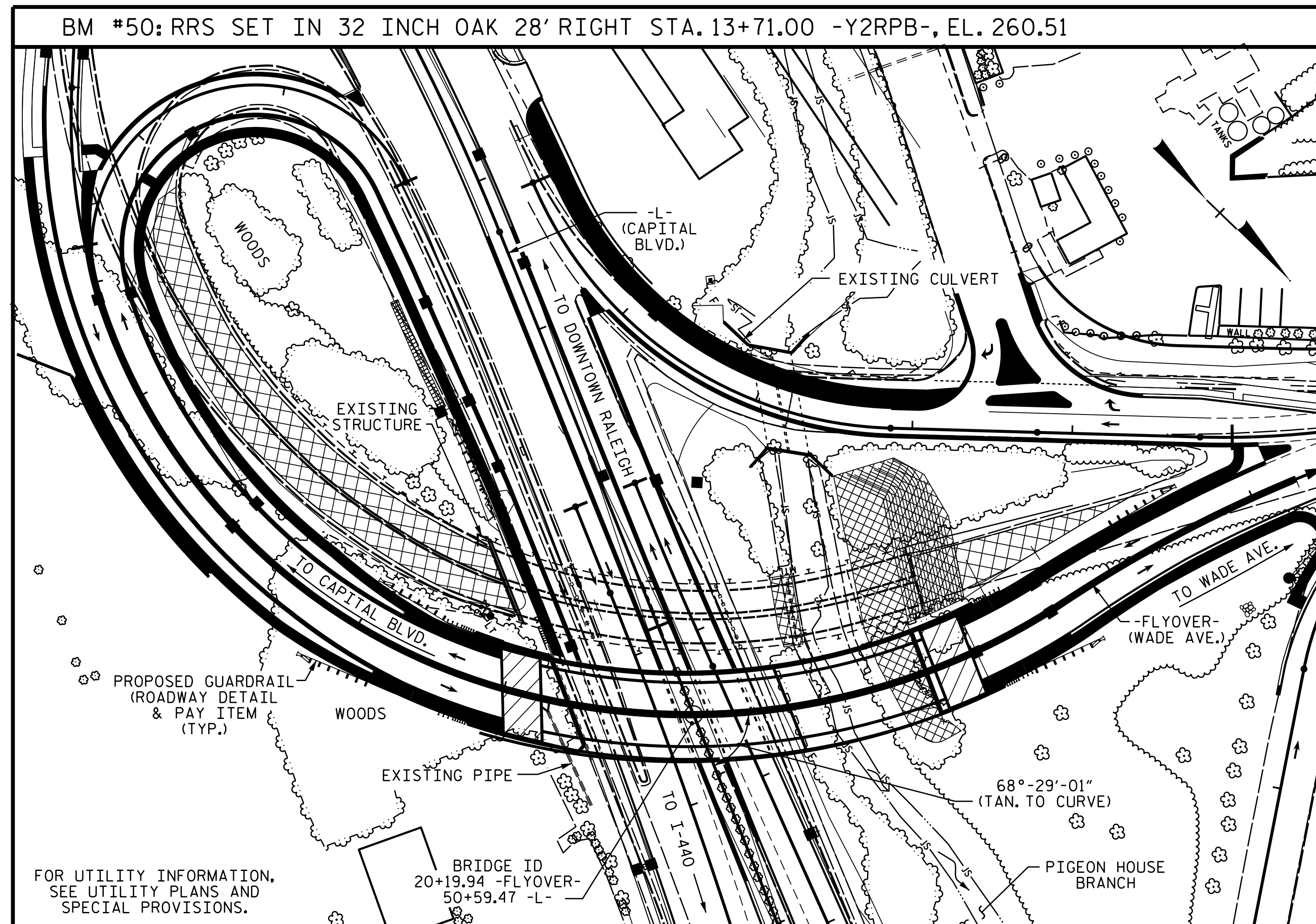
LOCATION SKETCH
