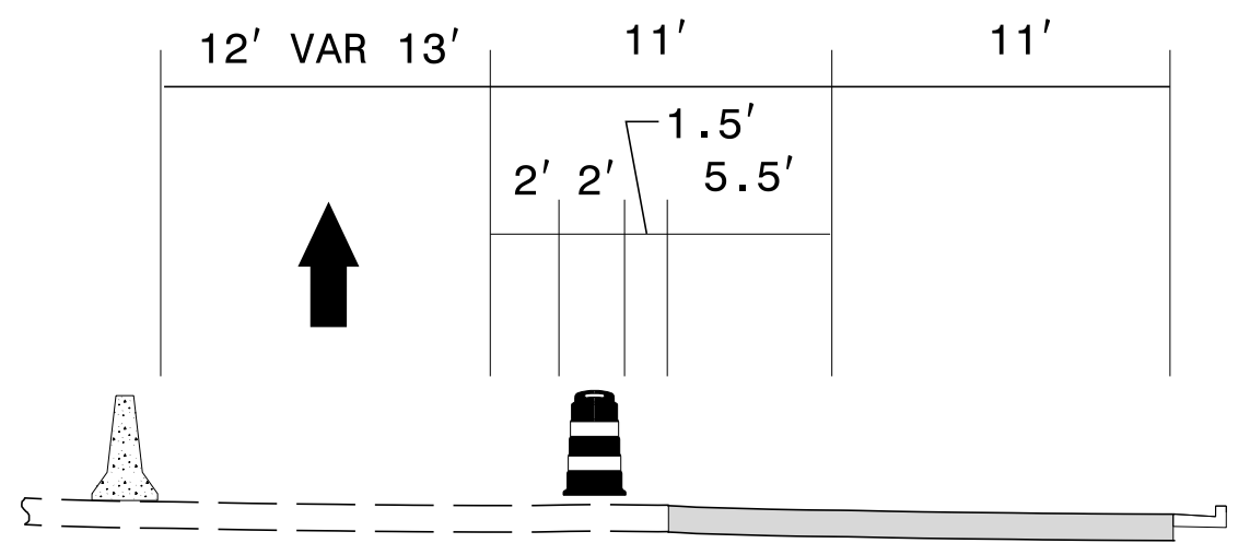
TYPICAL A-A REPLACE OUTSIDE 16.5'
