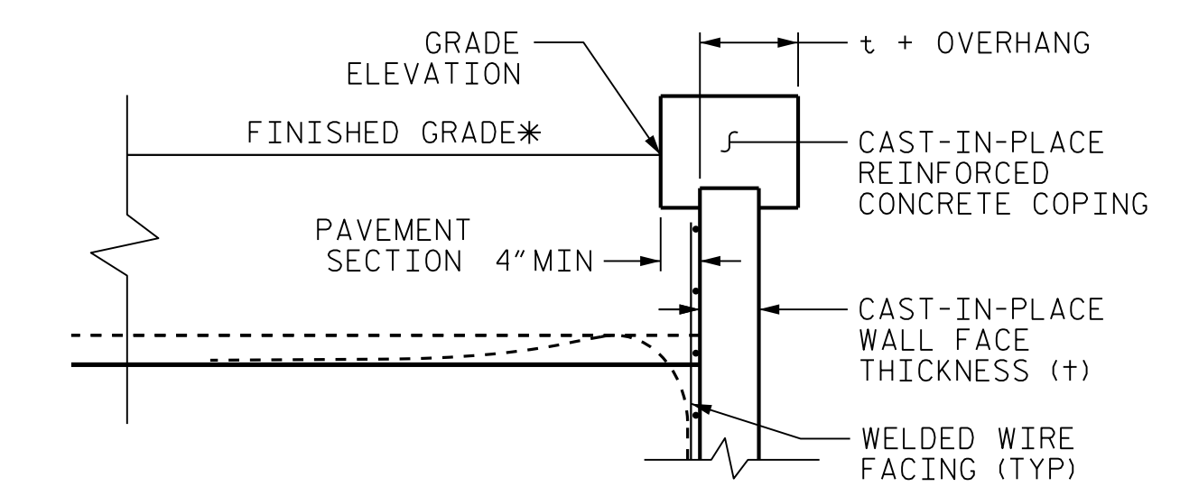
COPING DETAILS AT THE CONTRACTOR'S OPTION, CONNECT COPING TO PANELS WITH DOWELS OR EXTEND COPING DOWN BACK OF PANELS. *SEE ROADWAY PLANS FOR FINISHED GRADE DETAILS.
