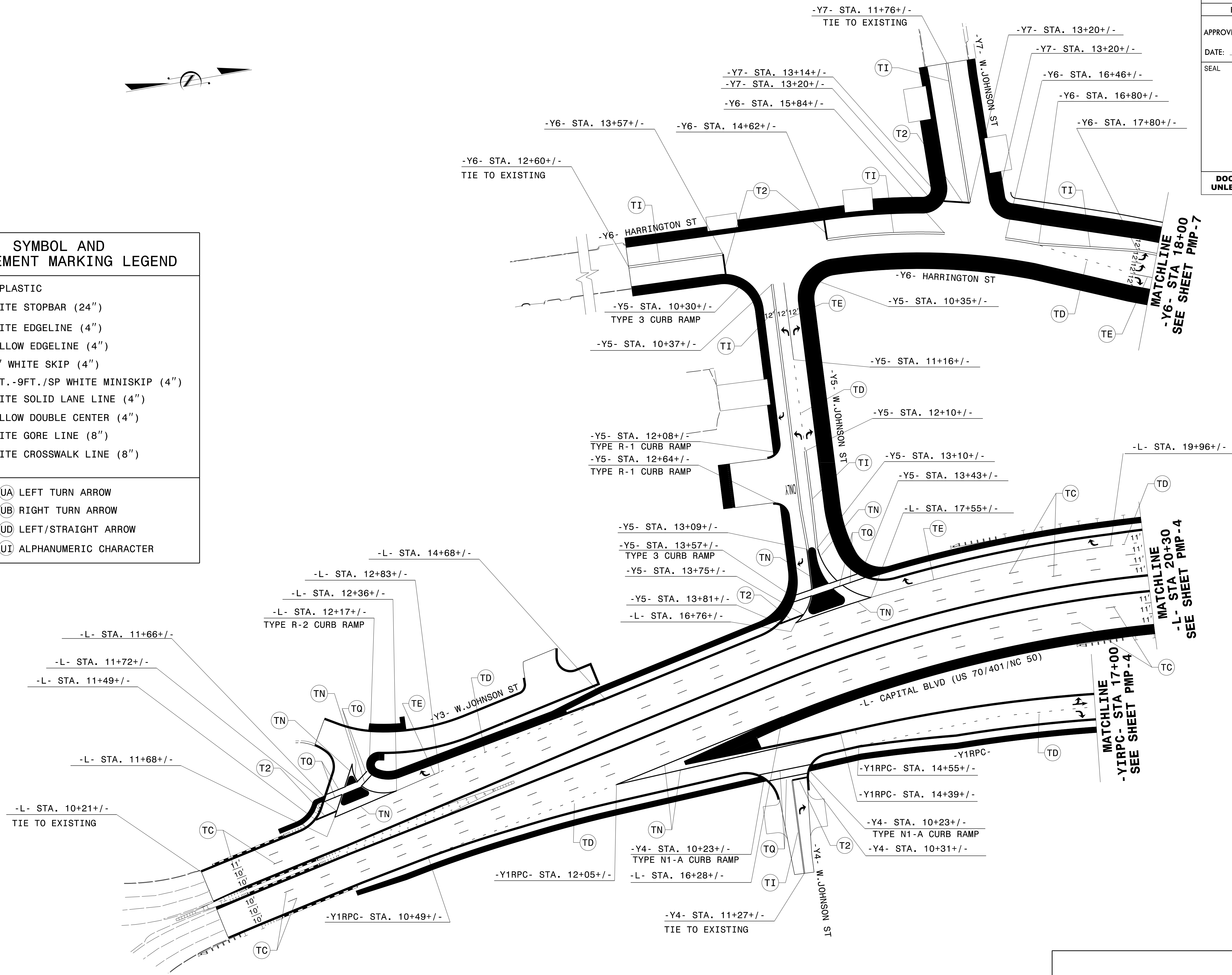
PAVEMENT MARKING DETAIL
